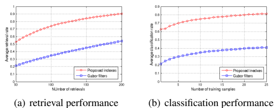
Figure 5: Average retrieval (a) and classification (b) performance.
