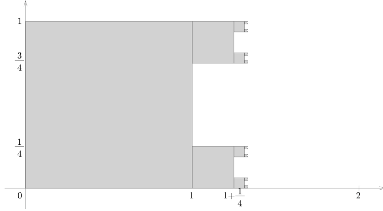
Figure 1: Fractal object
