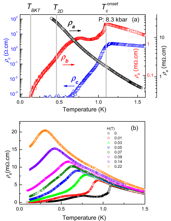
FIG. 4. (Color online) Phase B , P=8.3 kbar: (a) Temperature dependence of \rho_a , \rho_b and \rho_c . The line through the data points of \rho_b corresponds to the fit of \rho_b by the BKT model. (b) Temperature dependence of \rho_b for different magnetic fields.
