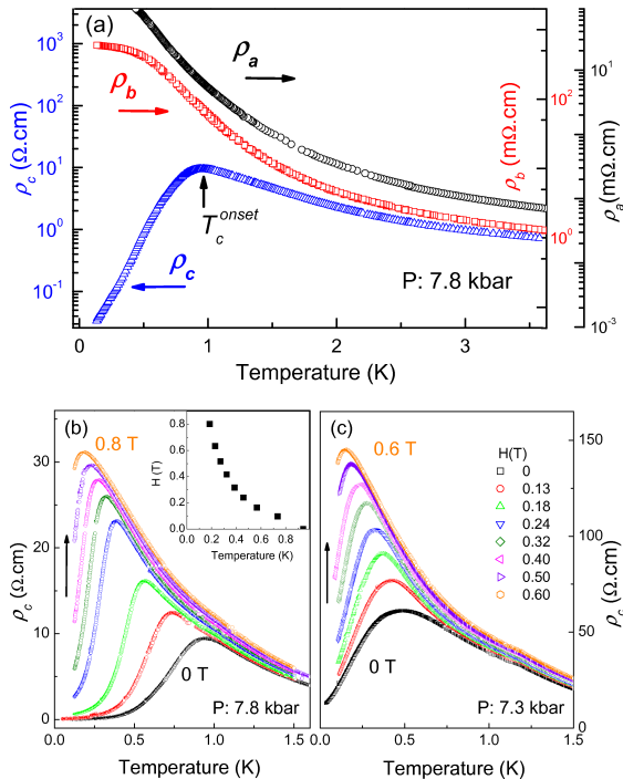
FIG. 2. (Color online) Phase A : (a) Temperature dependence of \rho_a , \rho_b and \rho_c at P = 7.8 kbar. (b) Temperature dependence of \rho_c at P = 7.8 kbar for magnetic fields ranging from 0 to 0.8T by step of 0.1T . The insert shows the deduced upper critical field line. (c) Temperature dependence of \rho_c at P = 7.3 kbar for different magnetic fields.
