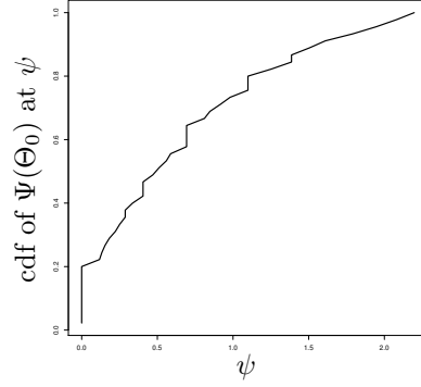
Figure 2: Cumulative distribution function \psi \mapsto \frac{1}{\#\Theta_0} \sum_{\theta \in \Theta_0} \mathbb{1}\{\Psi(\theta) \leq \psi\} of \Psi(\Theta_0) .
