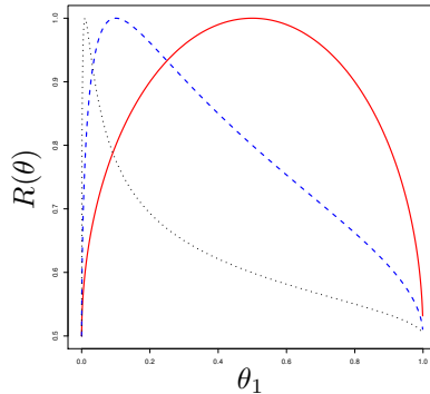
Figure 1: Plot of the relative efficiency R(\theta) as a function of \theta_1 for different values of \theta_0 ( \theta = (\theta_0, \theta_1) ). The solid, dashed and dotted curves respectively correspond to \theta_0 = \frac{1}{2}, \frac{1}{10}, \frac{1}{100} .
