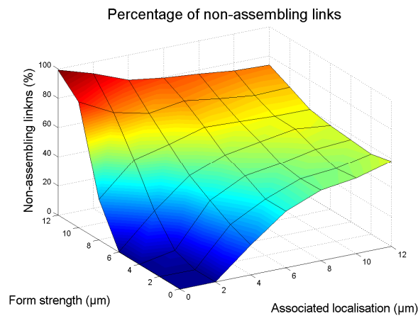
Fig. 9. Evolution of the rate of non-assembling linkages depending on the forms strengths and associated localisation for the 6\mu\text{m} linkage clearance value.
