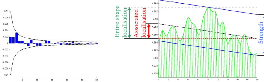
Fig. 4. a) randomly drawn modal signature, b) recombined shape, the least square associated geometry and the rectitude zone
