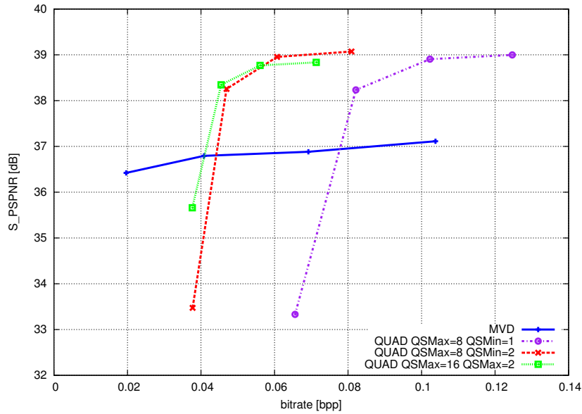
Figure 22. Rate distortion performance for view synthesis using MVD and quad-based approaches. Average bitrate VS average S_PSPNR for 2 intermediate views ( V_2 and V_4 ) and 25 frames of "Breakdancer" sequence.
