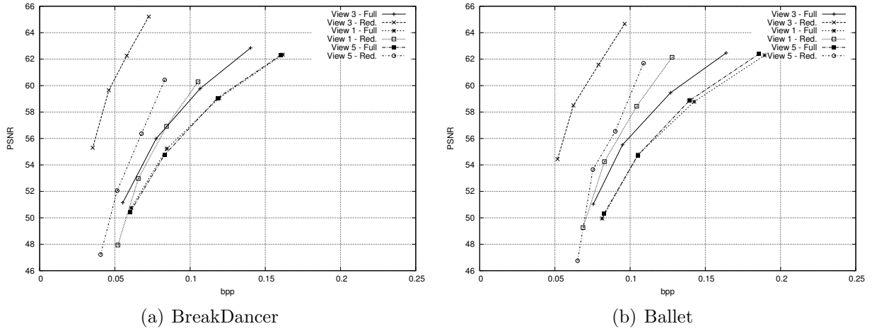
Figure 17. Rate distortion performance of reduced quadtree with respect to full quadtree for views 1, 3 and 5.
