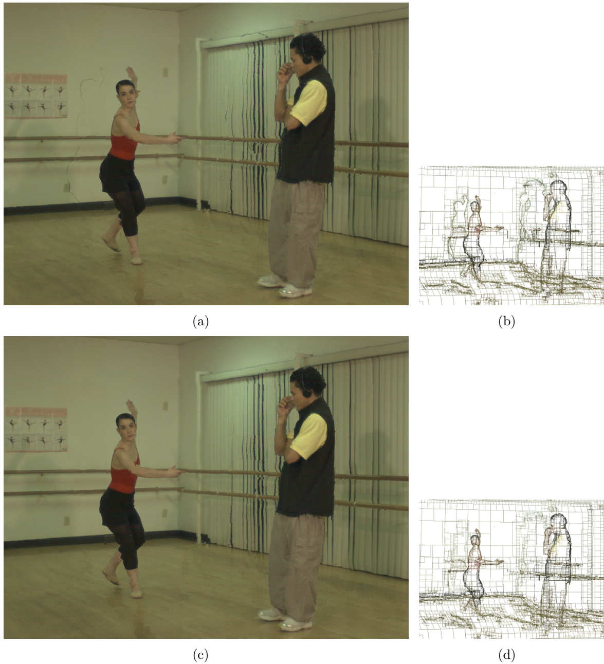
Figure 13. Effect of three step quad selection. (a) Synthesized view V_5 without redundancy reduction. (b) Corresponding quad representation. (c) Synthesized view V_5 with redundancy reduction. (d) Corresponding quad representation.
