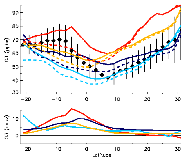
Fig. 5. Same as Fig. 4 but for O 3 .
