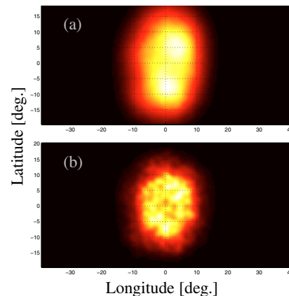
Fig. 6. RL iterations for the reconstruction of the disk with 1.5 \times 10^{-2} \text{ ph s}^{-1} \text{ cm}^{-2} : iteration number 3 a) and 13 b) .
