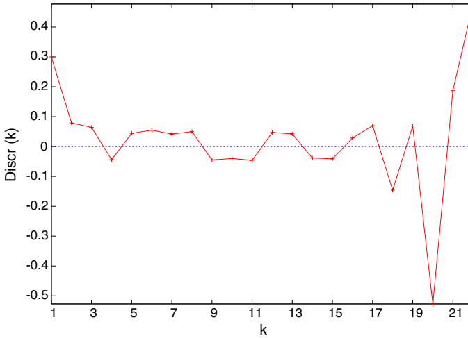
Fig. 1. Discrepancy \text{Discr} , as predicted by (5.11), vs wavenumber k for data obtained by spectral simulation in double precision; rounding noise becomes significant beyond wavenumber 17
