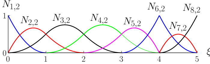
Fig. 2. Quadratic basis functions for an open, non-uniform knot vector \xi = \{0, 0, 0, 1, 2, 3, 4, 4, 5, 5, 5\}
