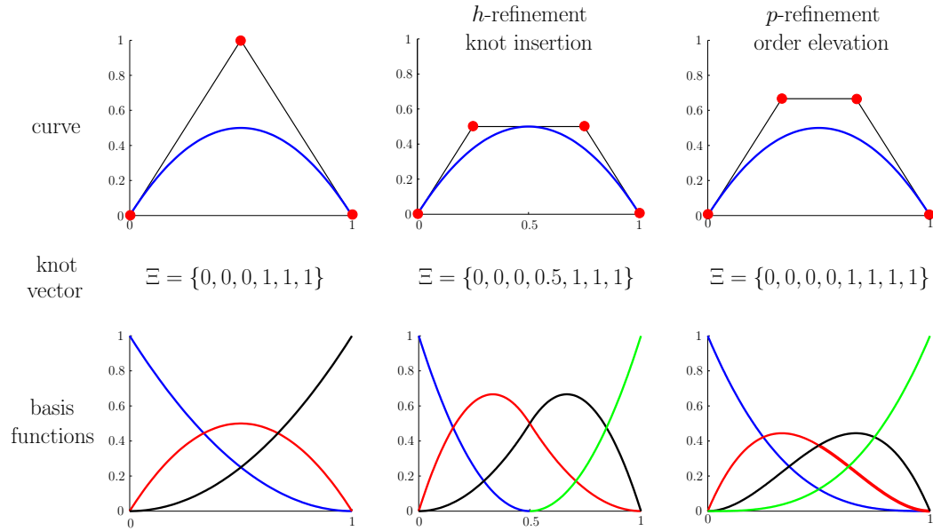
Fig. 4. Curve, control points, knot vectors and basis functions after knot insertion and order elevation of a quadratic curve. Control points are denoted by ●’s.
