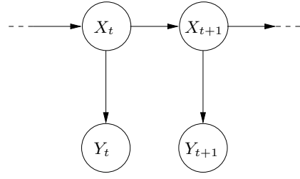
Fig. 1. Graphical representation of the dependence structure of an HMC
