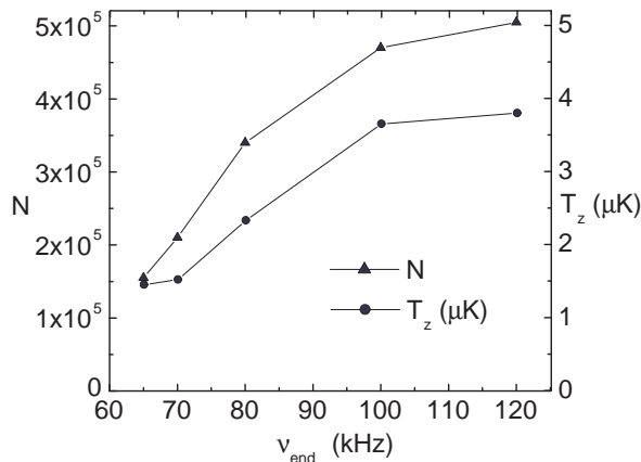
FIG. 7: Final atom number N and kinetic temperature T_z , deduced from the vertical size of the cloud after a time-of-flight expansion, after an evaporation ramp of the second RF field between 600 kHz and \nu_{\text{end}} .
