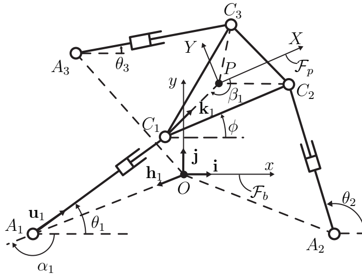
Figure 1. 3-RPR manipulator
