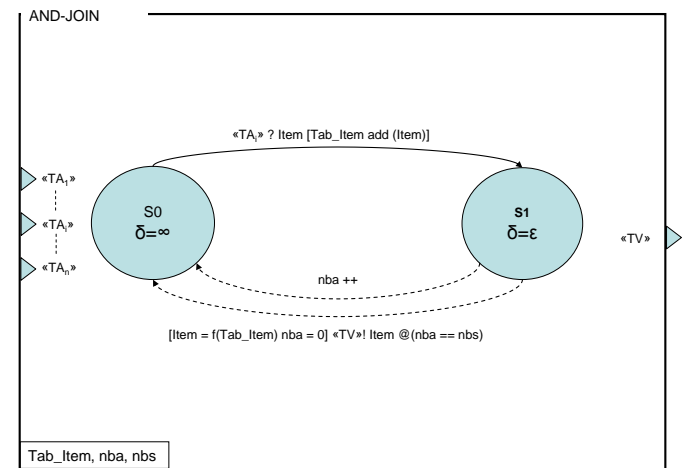
Fig. 13. G-DEVS AND-JOIN workflow block model
