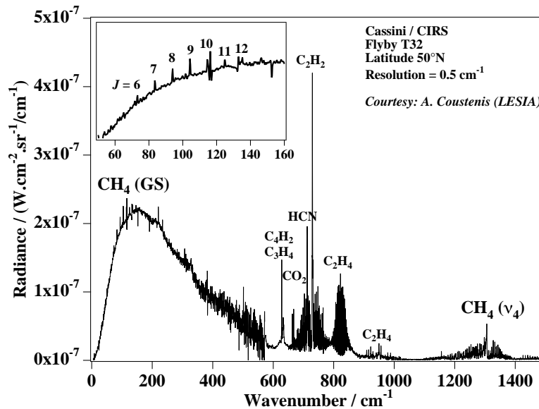
Figure 1: Example of a Cassini CIRS spectrum showing far infrared emission lines of methane.
