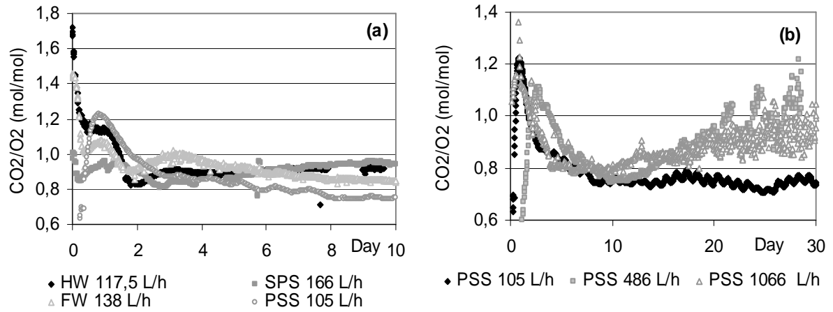
Figure 8: Variations of respiratory quotient for household waste, separated pig solids, food waste and pig slaughterhouse sludge.
