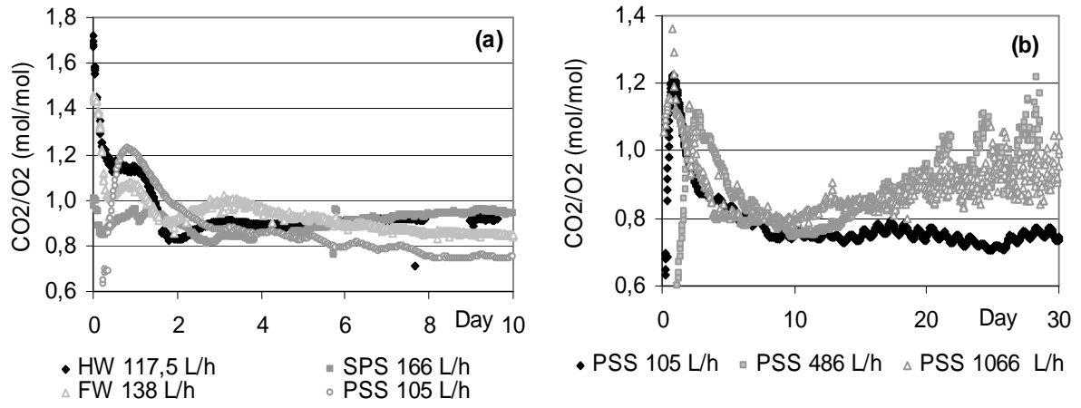
Figure 8: Variations of respiratory quotient for household waste, separated pig solids, food waste and pig slaughterhouse sludge.
