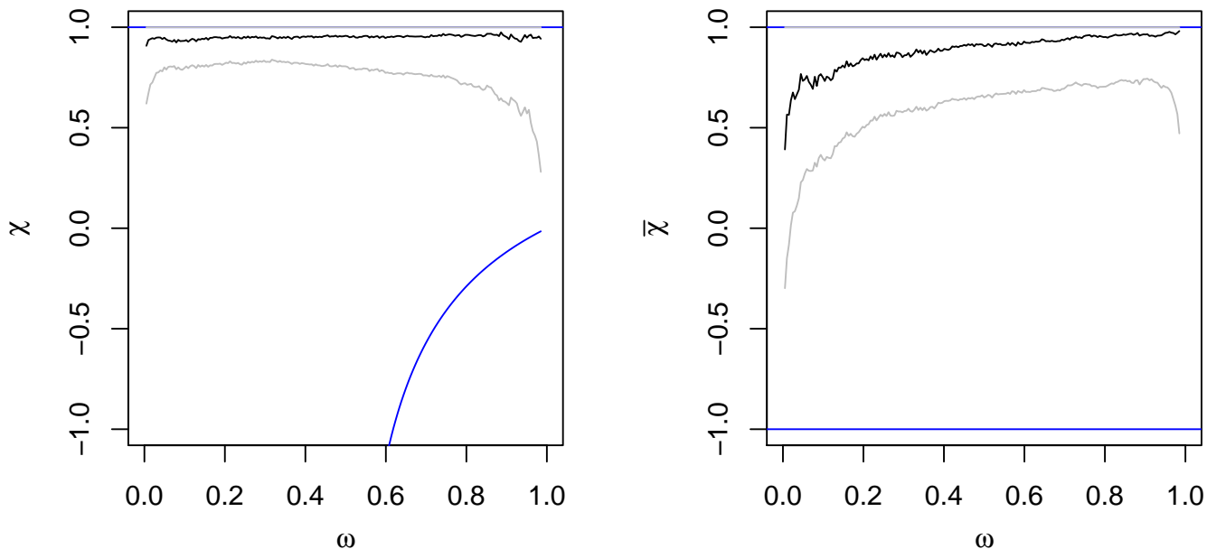
Figure 5: Plot of the \chi and \bar{\chi} statistics and the related 95% confidence intervals for station E6470910. The solid blue lines are the theoretical bounds.
