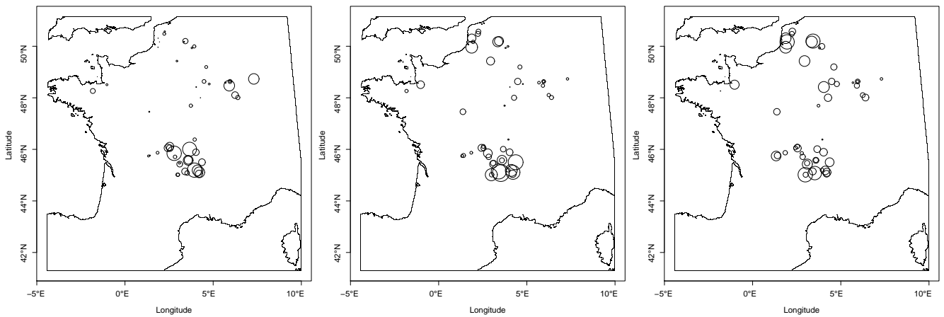
Figure 15: nmse spatial distribution according to the three Markovian models. Left panel: alog , middle panel: anlog and right panel: amix . The radius is proportional to the nmse value.
