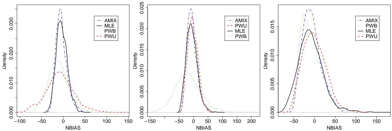
Figure 10: Densities of the normalized biases for the amix model and the MLE , PWU , and PWB estimators for quantiles Q_5 (left panel), Q_{10} (middle panel) and Q_{20} (right panel). Record length: 5 years.
