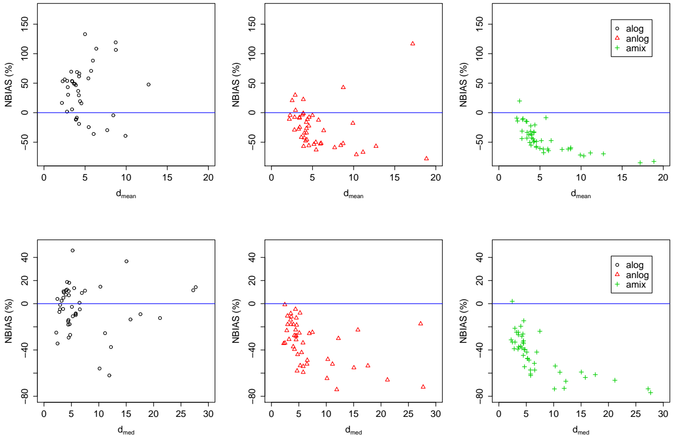
Figure 12: d_{mean} and d_{med} normalized biases as a function of the theoretical values for the three asymmetric Markovian models.
