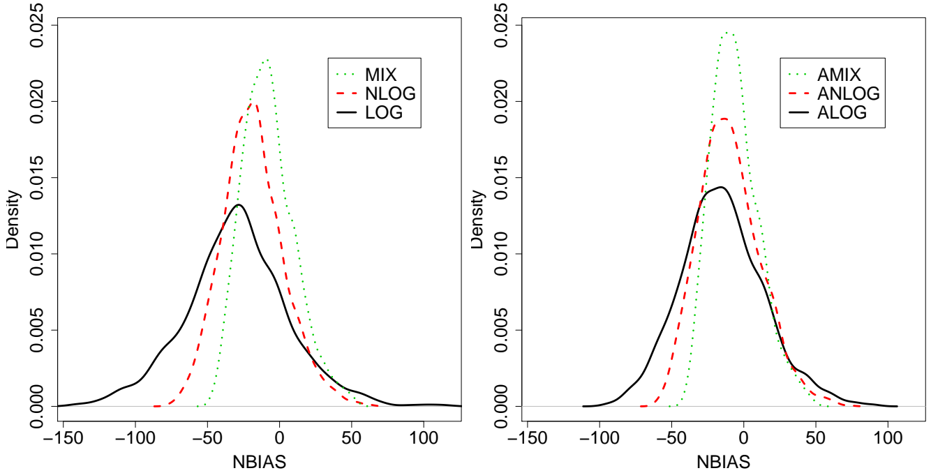
Figure 8: Densities of the normalized biases of Q_{20} estimates for the symmetric Markovian models (left panel) and the asymmetric ones (right panel). Target site record length: 5 years.
