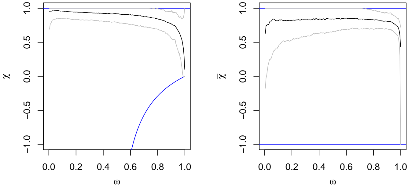
Figure 6: Plot of the \chi and \bar{\chi} statistics and the related 95% intervals for station A4200630. The solid blue lines are the theoretical bounds.
