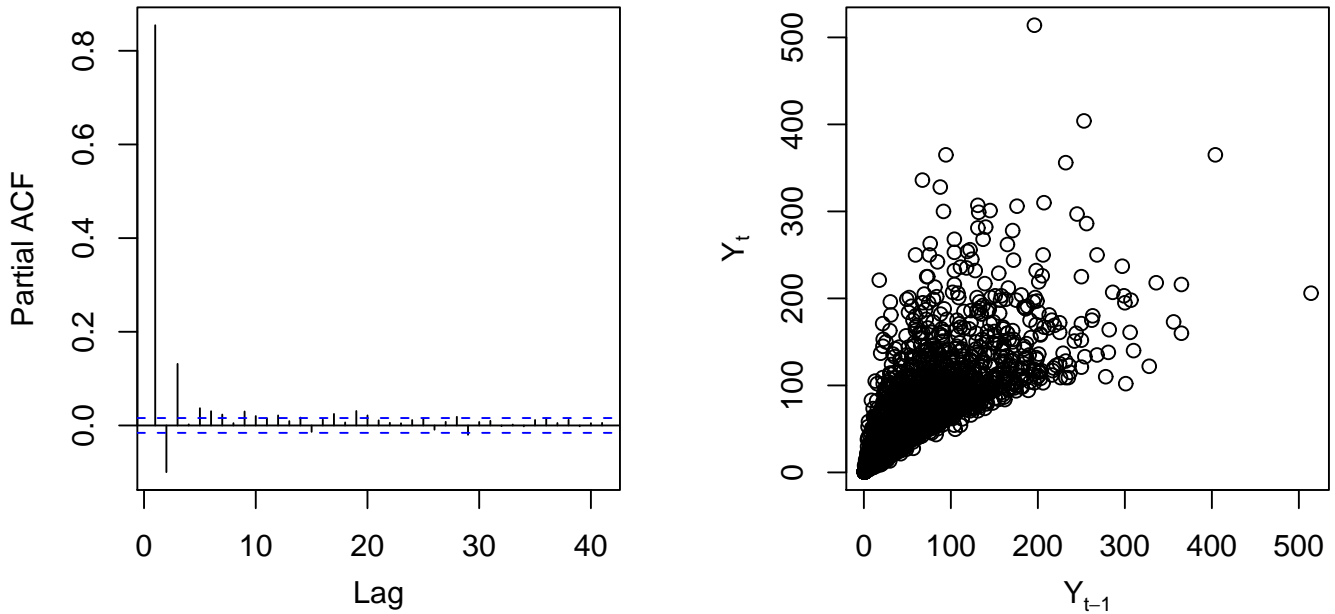
Figure 3: Autocorrelation plot (left panel) and scatterplot of the time series at lag 1 (right panel) for station A4200630.
