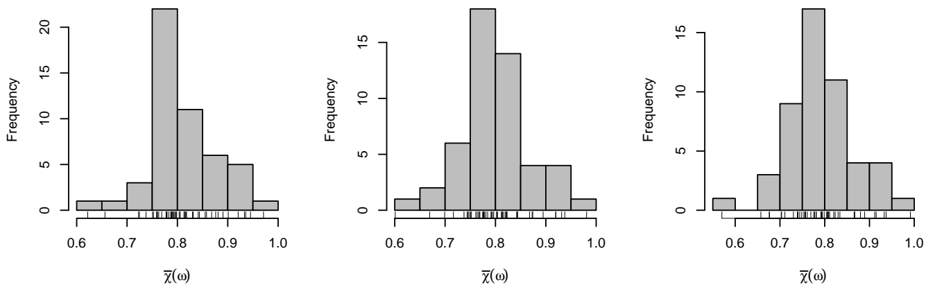
Figure 7: Histograms of the \bar{\chi}(\omega) statistics for different \omega values. Left panel: \omega = 0.98 , middle panel: \omega = 0.985 and right panel: \omega = 0.99 .
