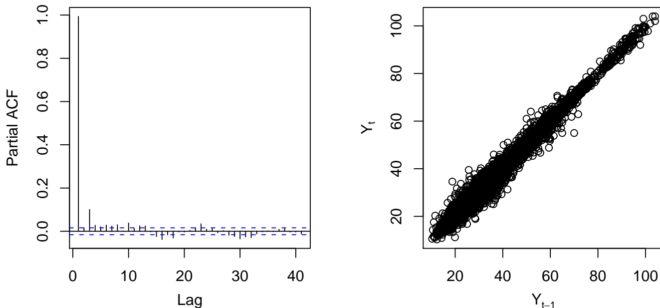
Figure 2: Autocorrelation plot (left panel) and scatterplot of the time series at lag 1 (right panel) for station E6470910.
