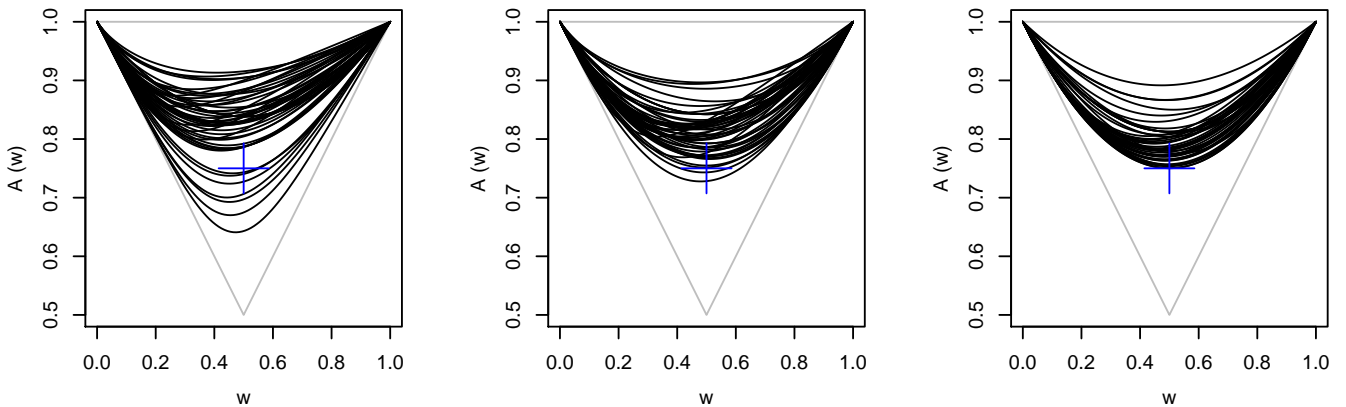
Figure 9: Representation of the Pickands dependence functions for the 50 gaging stations. Left panel : alog , middle panel: anlog and right panel: amix . “+” represents the theoretical dependence bound for the amix model.
