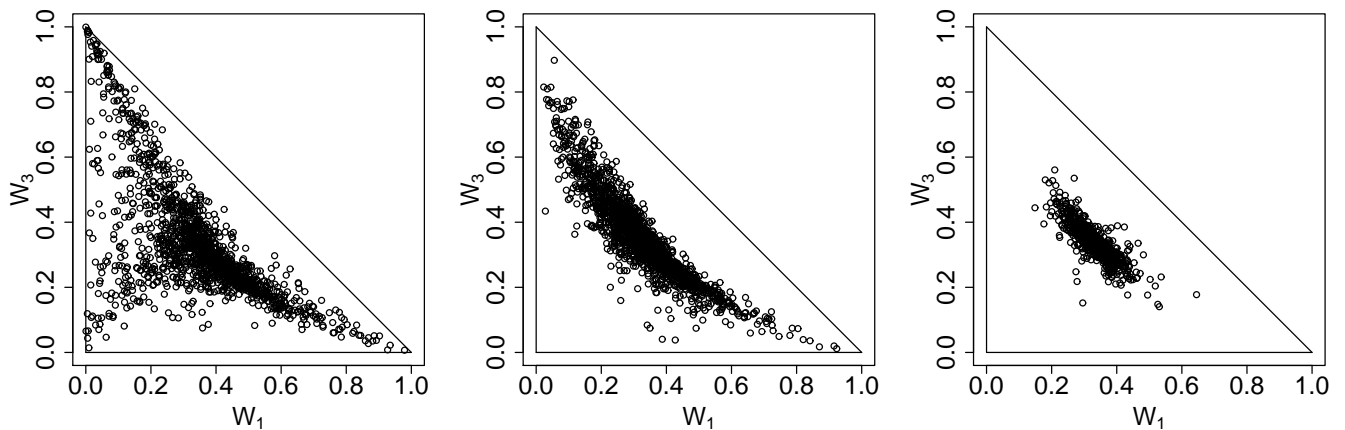
Figure 4: Simplex plots for stations K0523010 (left panel), K4470010 (middle panel) and E6470910 (right panel).
