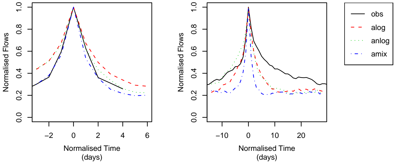
Figure 13: Observed and simulated normalized mean hydrographs for the J0621610 (left panel) and the L0400610 (right panel) stations.
