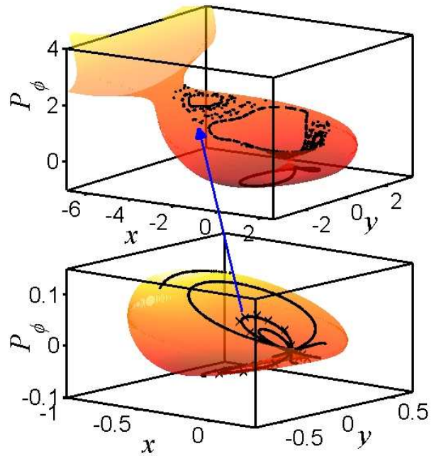
FIG. 3: Poincaré sections of the inner electron reduced model in the 3D space (x, y, P_\phi = xp_y - yp_x) . The admissible set is represented by the surface and Poincaré sections are represented by dots. Lower panel: Sections for a Jacobi constant \mathcal{K} = -0.659 which corresponds to the constant for the inner electron in Fig. 2 when it is close to the nucleus and the outer electron is far away. For comparison, we display the Poincaré section associated with this part of the trajectory for the full model (crosses). Upper panel: Poincaré surface for a Jacobi constant \mathcal{K} = -0.5 , when the ionization channel is open. The arrow represents the jump, from an invariant torus up to the chaotic unbounded area, experienced by the inner electron during NSDI.
