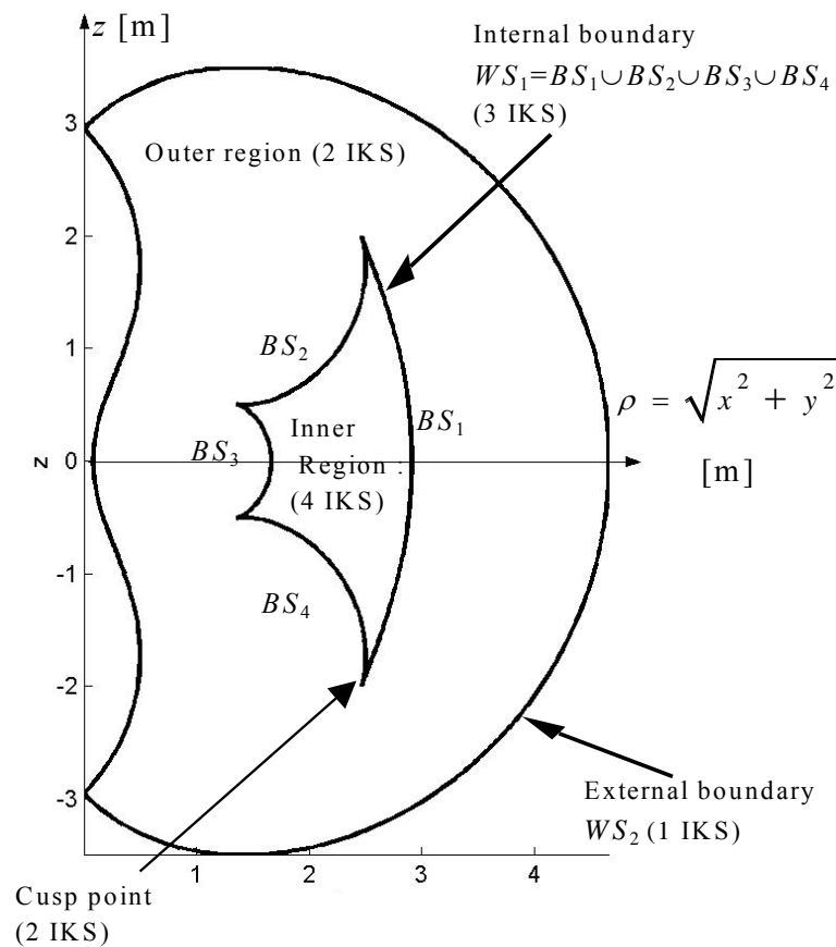
Fig. 3. Singularity locus in workspace. Number of distinct inverse kinematic solutions (IKS) in each region and on each boundary is indicated.
