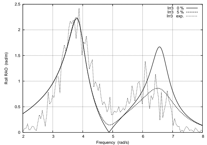
Figure 7. ROLL RAO. FLAT ROOF 16 CM ABOVE STILL WATER LEVEL. SEASTATE IRR3.
