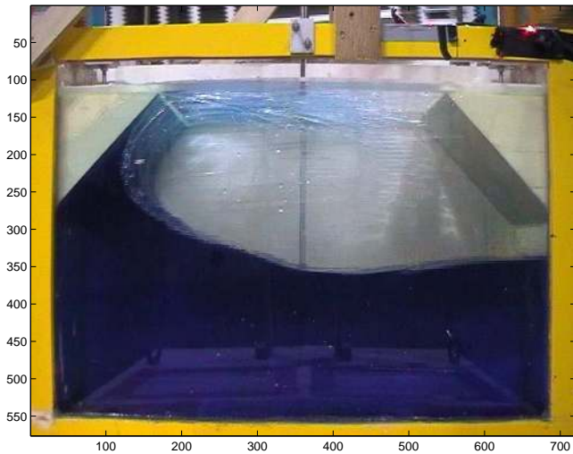
Figure 12. CHAMFERS IN P45 CONFIGURATION. VIEW FROM THE ONBOARD VIDEO CAMERA.
