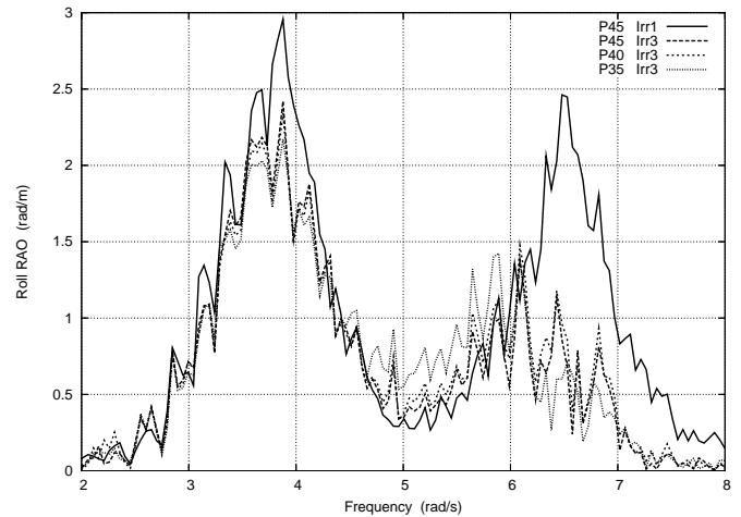
Figure 10. ROLL RAO FOR DIFFERENT ROOF ELEVATIONS.
