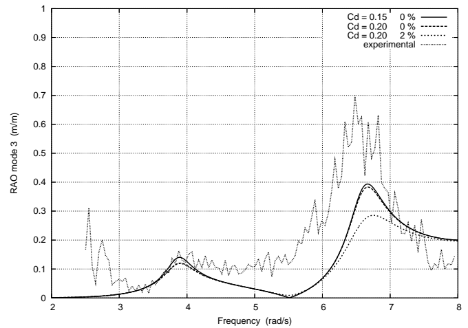
Figure 6. RAO OF THE SECOND ODD MODE. FLAT ROOF 16 CM ABOVE STILL WATER LEVEL. SEASTATE IRR1.
