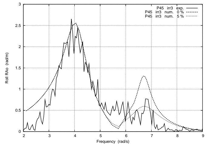
Figure 14. CONFIGURATION P45. SEASTATE IRR3. MEASURED AND CALCULATED ROLL RAOS.
