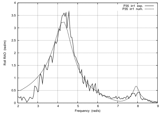
Figure 17. CHAMFERS AT 12 CM IMMERSION. SEASTATE IRR1. MEASURED AND CALCULATED ROLL RAOS.
