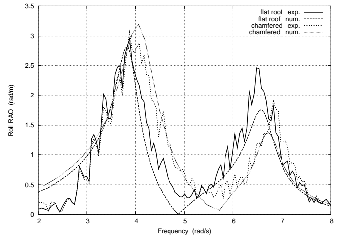
Figure 13. CONFIGURATION P45. SEASTATE IRR1. MEASURED AND CALCULATED ROLL RAOS.
