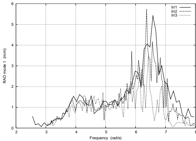
Figure 8. RAO OF THE FIRST SLOSHING MODE. FLAT ROOF 16 CM ABOVE STILL WATER LEVEL. SEASTATES IRR1, IRR2, IRR3.
