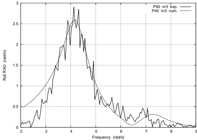
Figure 16. CHAMFERS 7 CM IN WATER. SEASTATE IRR3. MEASURED AND CALCULATED ROLL RAOS.
