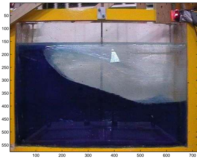
Figure 9. FLAT ROOF IN P40 CONFIGURATION. VIEW FROM THE ONBOARD VIDEO CAMERA (NUMBERS ARE PIXELS).
