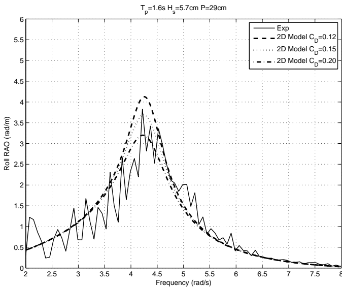
Figure 2. CLOSED TANKS. EXPERIMENTAL AND NUMERICAL ROLL RAOs. SEASTATE IRR1.
