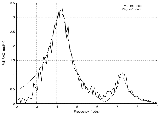
Figure 15. CHAMFERS 7 CM IN WATER. SEASTATE IRR1. MEASURED AND CALCULATED ROLL RAOS.
