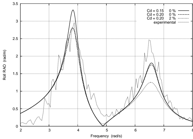
Figure 4. ROLL RAO. FLAT ROOF 16 CM ABOVE STILL WATER LEVEL. SEASTATE IRR1.
