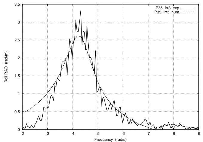
Figure 18. CHAMFERS AT 12 CM IMMERSION. SEASTATE IRR3. MEASURED AND CALCULATED ROLL RAOS.
