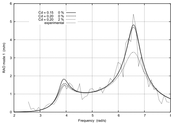
Figure 5. RAO OF THE FIRST SLOSHING MODE. FLAT ROOF 16 CM ABOVE STILL WATER LEVEL. SEASTATE IRR1.
