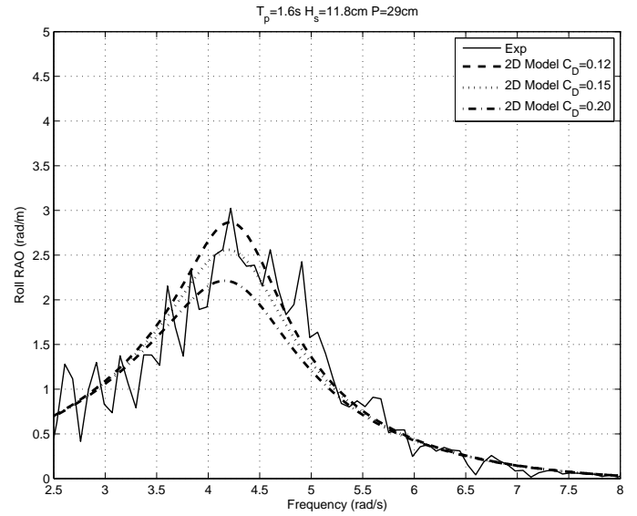
Figure 3. CLOSED TANKS. EXPERIMENTAL AND NUMERICAL ROLL RAOs. SEASTATE IRR3.
