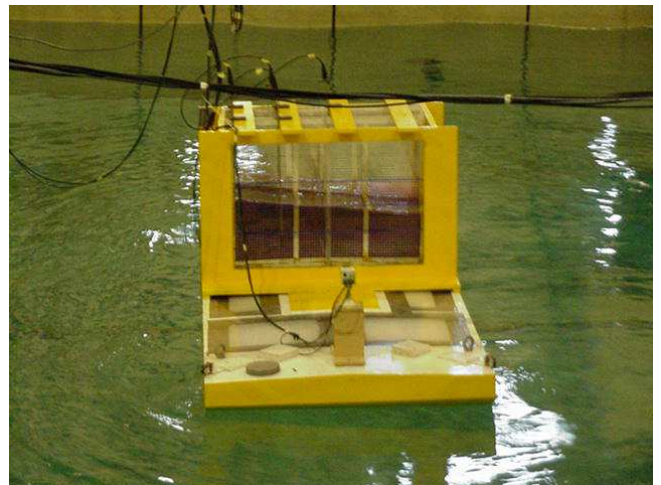
Figure 1. BARGE MODEL IN THE BASIN (FROM [1]).
