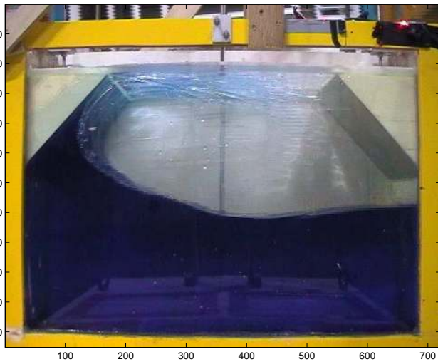
Figure 12. CHAMFERS IN P45 CONFIGURATION. VIEW FROM THE ONBOARD VIDEO CAMERA.
