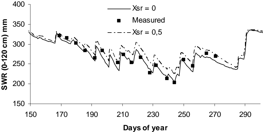
Fig. 4 Mulching impact on the soil water reserve ( SWR ) evolution according to PILOTE on the climatic scenario of 1999 for corn ( Samsara variety; T1 in conventional tillage: X_{sr} = 0 ; CE = 0.92 , RMSE = 9.0 mm))
