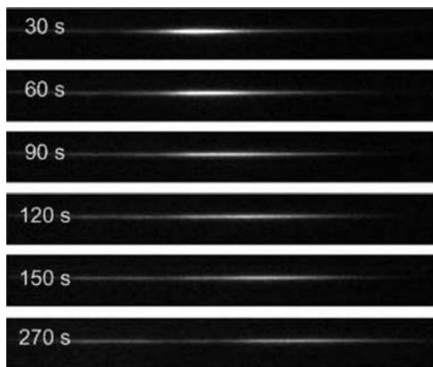
Fig. 3. Slow temporal evolution of the output beam in the nonlinear regime of propagation. These results were obtained at \lambda=1.53 \mu\text{m} . At t=0 \text{ s} (not shown), the output beam profile matches the input beam as in Figs. 2(a), 2(c), and 2(g).
