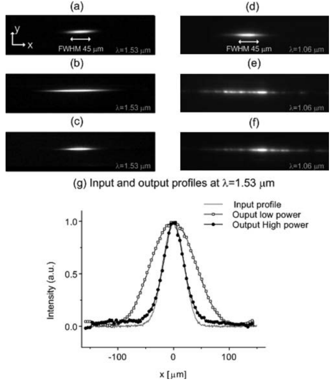
Fig. 2. Experimental results showing both soliton beam formation and self-focusing at (a), (b), (c) \lambda=1.53 \mu\text{m} and (d), (e), (f) \lambda=1.06 \mu\text{m} in \text{Ge}_{25}\text{Sb}_{10}\text{S}_{65} and \text{Ge}_{15}\text{Sb}_{20}\text{S}_{65} chalcogenide slab waveguides, respectively. (a), (d) Laser beam profile at the input of the guiding structure. (b), (e) Output beam profile at low power and (c), (f) in the nonlinear regime of propagation at a peak intensity of 1 \text{ GW}/\text{cm}^2 . (g) Intensity profiles corresponding to Figs (a)–(c).
