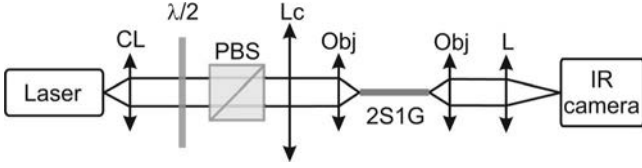
Fig. 1. Experimental setup for the study of bright Kerr solitons in slab chalcogenide waveguides. CL, collimating lens; \lambda/2 , half-wave plate; PBS, polarizing beam splitter; L_c , cylindrical lens; Obj, microscope objective; 2S1G, slab waveguide; L, lens. The laser source is either a 1.06 \mu\text{m} Nd:YAG, 700 ps pulse duration microchip laser or a 1.53 \mu\text{m} , 5 ps amplified fiber laser.
