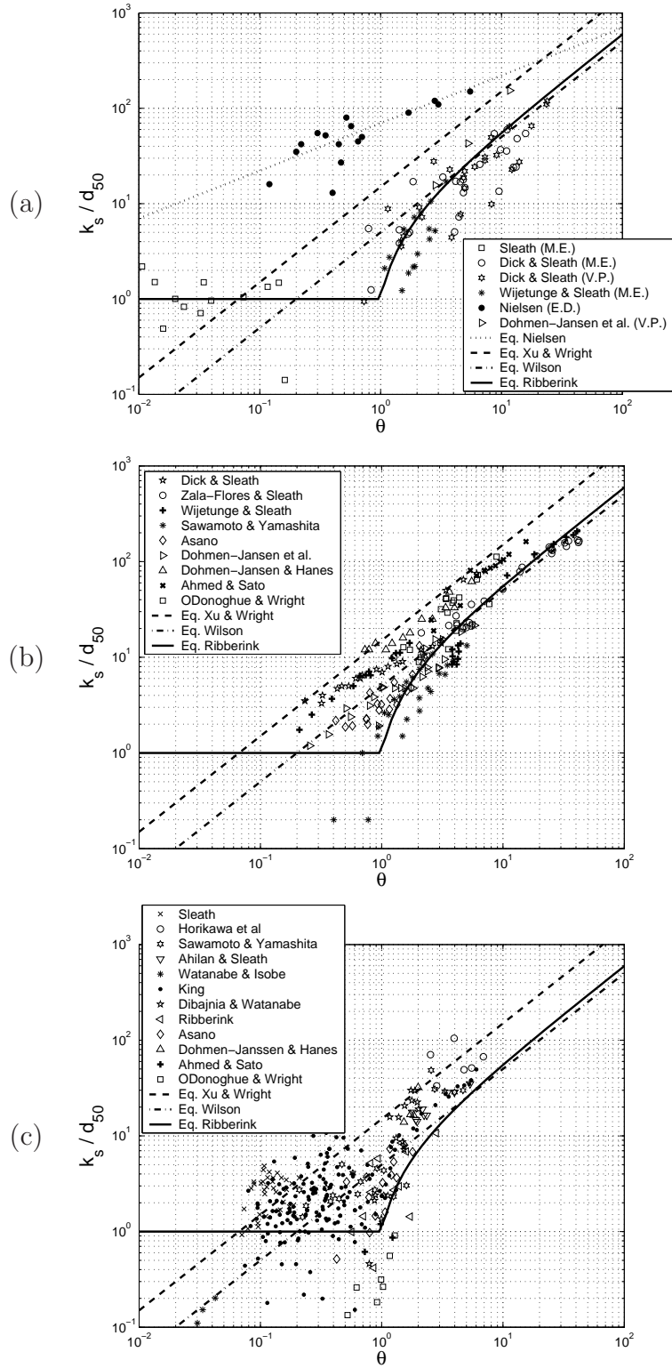
Figure 4: Effective roughness ratio versus total Shields parameter, together with semi-empirical predictive relationships, including data obtained using (a) the “velocity profile” (V.P.), “momentum equation” (M.E.) and “energy dissipation” (E.D.) methods; (b) the “sheet flow layer” method; and (c) the “bed-load transport” method.
