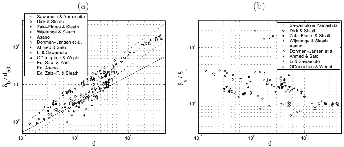
Figure 2: (a) Erosion thickness \delta_b and (b) the ratio \delta_s/\delta_b versus the total Shields parameter calculated using the relationship k_s = \delta_b .
