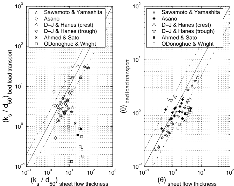
Figure 3: Validation of the “bed-load transport” method against the “sheet flow thickness” method (solid line corresponds to a perfect agreement, dashed lines to an agreement within a factor 2).
