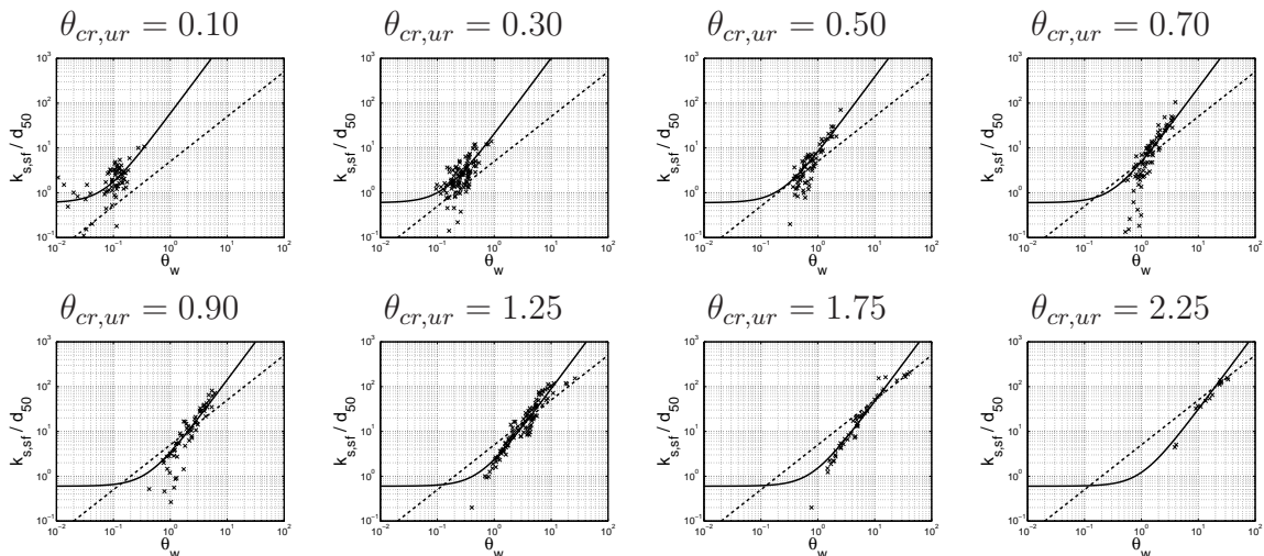
Figure 7: Dimensionless roughness height versus Shields parameter for different values on the critical Shields parameter for the upper regime (the bold lines correspond to Eq. 33 and the dashed lines to the Wilson formula, Eq. 3).
