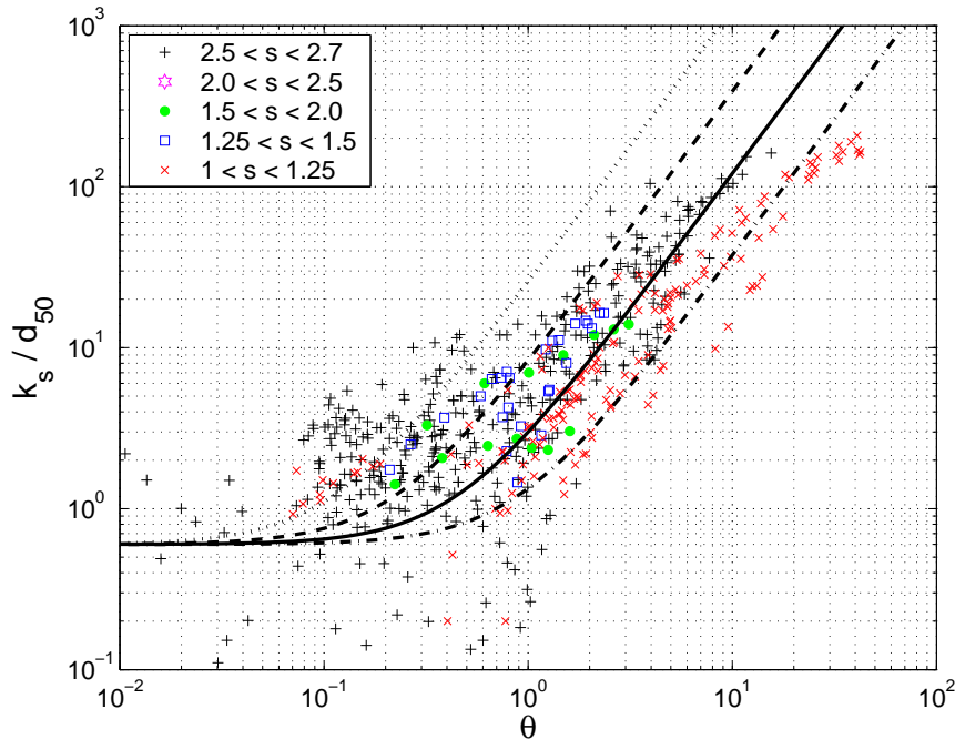
Figure 5: The effective roughness ratio versus the total Shields parameter (using all data apart from the “energy dissipation” method) including the influence of sediment density (the dotted, dashed, solid, and dashed-dotted lines correspond to Eq. 33 with a = 0.6 and b = 2.4 , and \theta_{cr,ur} = 0.25, 0.5, 1.0 and 2.0 , respectively).
