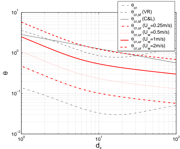
Figure 8: Comparison between the critical Shields parameter for the upper regime and critical Shields parameters for the inception of sheet flow (VR: Van Rijn, 1993; C&L: Camenen & Larson,).
