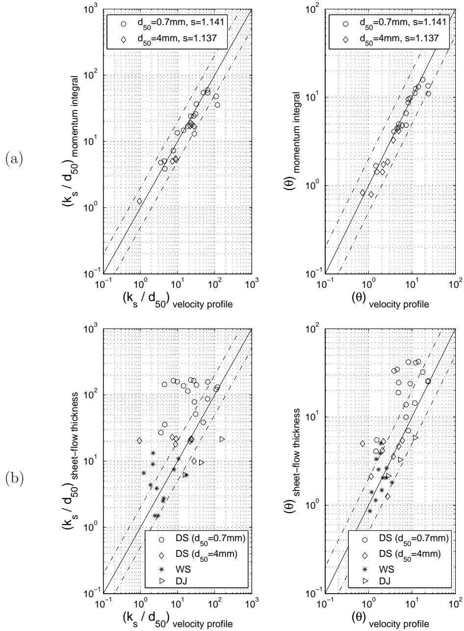
Figure 1: Validation of the “momentum equation” method (a) and “sheet flow thickness” method (b) against the “velocity profile” method (solid line corresponds to a perfect agreement, dashed lines to an agreement within a factor 2; data from Dick & Sleath, 1991 in (a); DS: Dick & Sleath, 1991, WS: Wijetunde & Sleath, 1998, DJ: Dohmen-Jansen et al. , 2001 in (b)).
