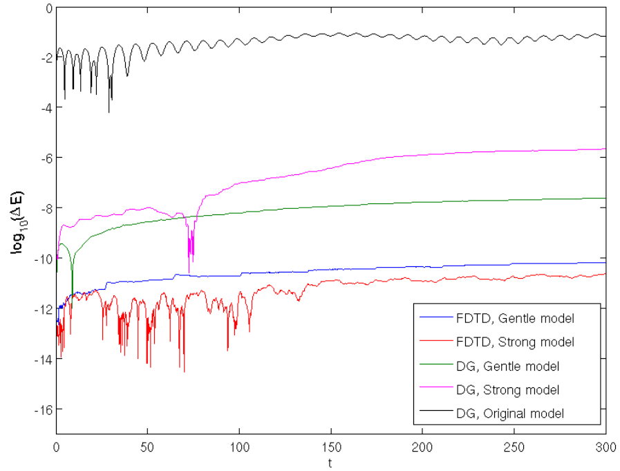
FIGURE 8. Logarithm of variation of energy versus time for gentle scheme, strong scheme and original scheme for solitary-wave and sinusoidal bottom ( c_1 = 0.5 , \mu = 0.05 , \varepsilon = \sqrt{\mu} , \alpha = 0.5\varepsilon , \beta = \varepsilon ) Finite difference and fourth order LDG with 5120 degrees of freedom.
