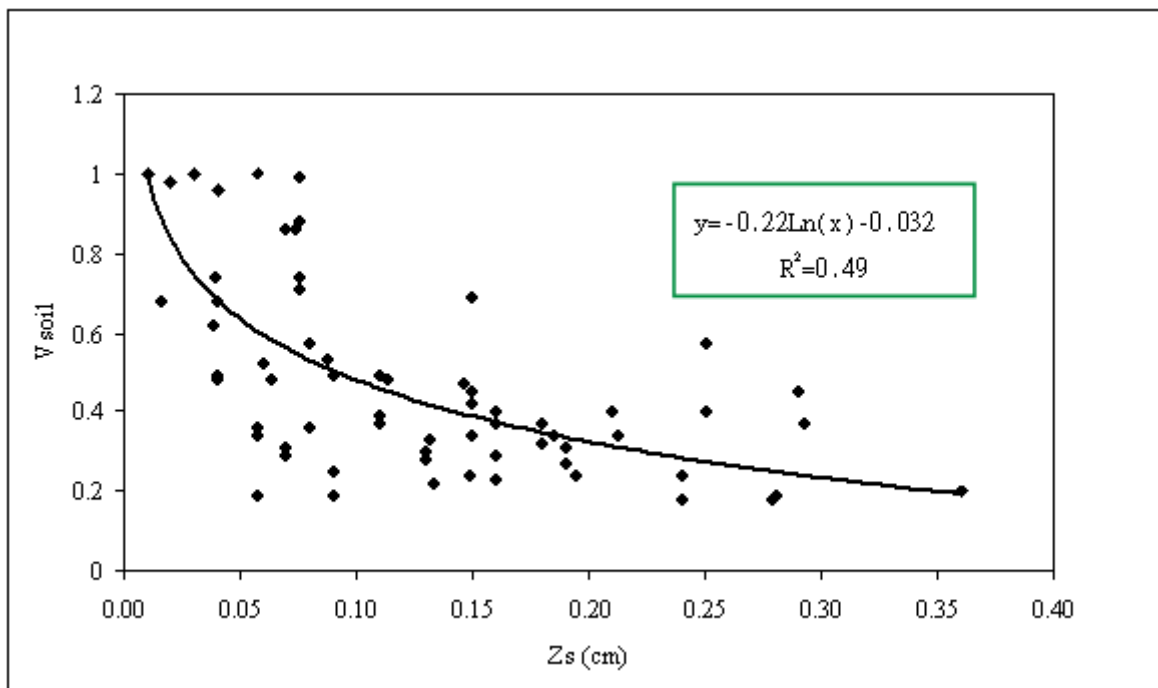
Figure 5. Variation of the v_{soil} parameter (soil fraction) as a function of the soil roughness parameter Z_s .
