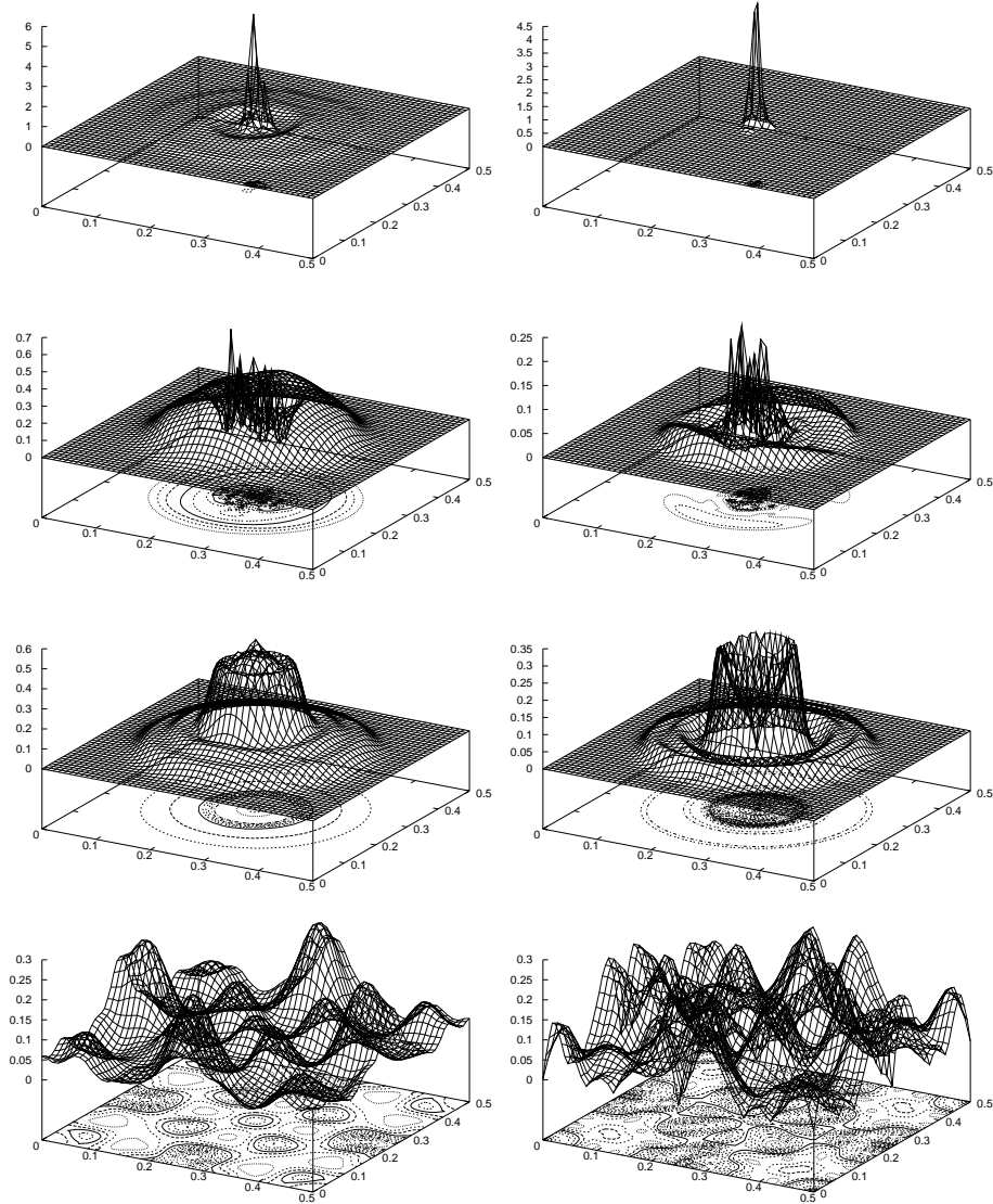
FIGURE 18. Position (left column) and current density (right column) at T = 0.15 sec for (resp. from the top) \varepsilon = 0, 0.001, 0.01 and 0.1 nearly after the solution blows up for \varepsilon = 0 .
