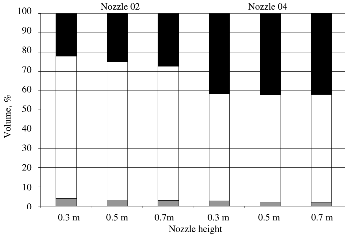
Fig. 5. Granulometry of the nozzles at several heights: grey, 0-150 μm; white, 150-400 μm; black, >400 μm
