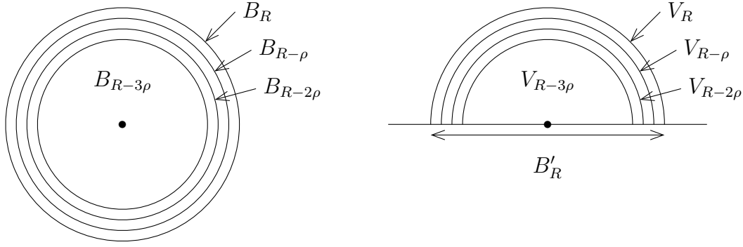
Figure 2.4: Nested neighborhoods (balls and half-balls)
