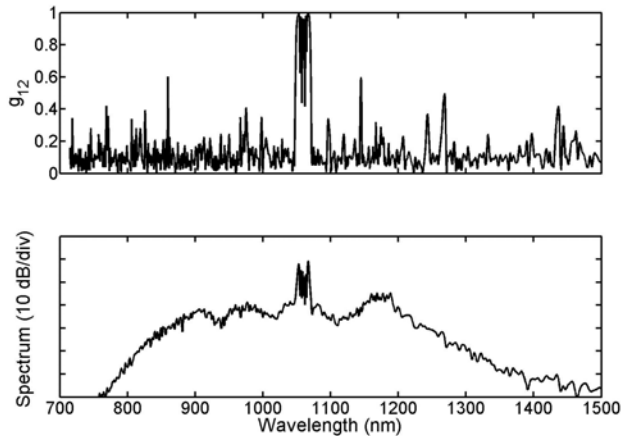
Fig. 1 Top: coherence and bottom: averaged SC spectrum generated in the unmodulated case.
