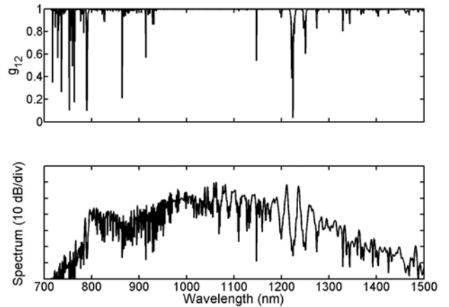
Fig. 2 Top: coherence and bottom: averaged SC spectrum generated when the input pulse is modulated.
