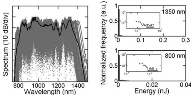
Fig. 4. Left, individual results from simulation ensemble (gray; for clarity only 50 individual shots are plotted) with calculated mean (solid). Right, energy histogram for filter cutoff wavelengths at 1350 and 800 nm. Insets, histograms in log-log scale.
