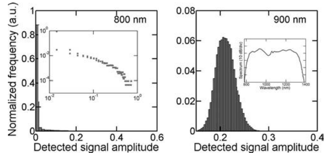
Fig. 3. Histogram of photodiode signal amplitude illustrating the blue edge fluctuations in the SC spectrum. The corresponding SC and the histogram in log-log scale are shown as insets. Spectral filtering at (left) 800 and (right) 900 nm.
