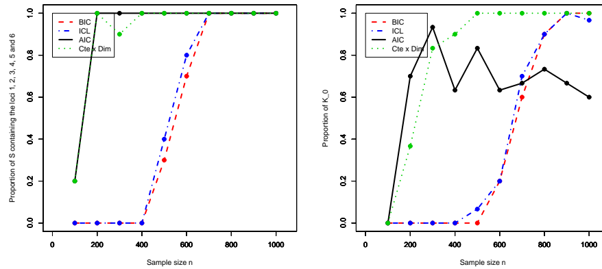
FIG 2. Left: Graph showing the proportion of selected models with \widehat{S}_n containing 1, ..., 6 with respect to sample size n . Right: Graph showing the proportion of selected models with \widehat{K}_n = K_0 with respect to sample size n .
