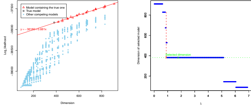
(a) \hat{\lambda}_{\min} \approx 0.88 by linear regression on sub-models. (b) The biggest jump occurs around 5.10, but the sliding window selects the more reasonable value \lambda_{\min} \approx 0.9 .
