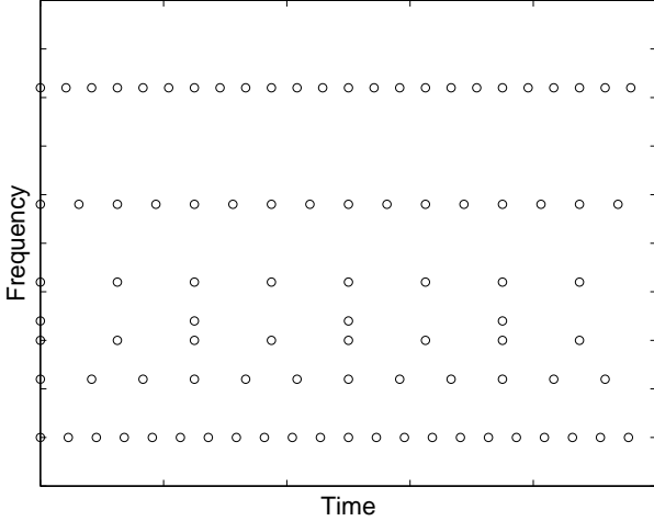
Figure 3: Example of sampling grid of the time-frequency plane when building a decomposition with time-frequency resolution evolving over frequency.
