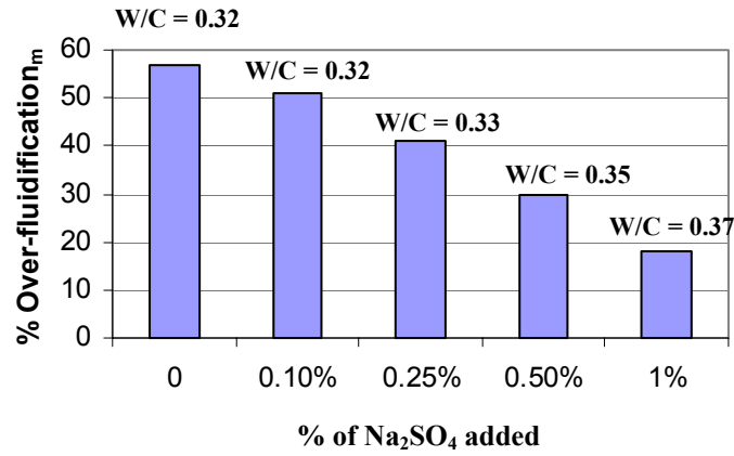
Fig. 10: Influence of the quantity of Na 2 SO 4 added on the % of over-fluidification m (see equation 2): Cement paste with Clinker L 50/50m gypsum/hemi- hydrate, PCP ref = 0.16%, W/C adjusted to get the same initial viscosity, Initial mixing: 1 min, 80 s -1 , T = 20°C
