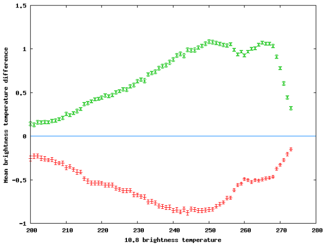
Fig. 2a. Difference of the mean value of 08.7\ \mu\text{m} and 12.0\ \mu\text{m} channels between non rainy and rainy pixels plotted versus 10.8\ \mu\text{m} brightness temperature in red and green respectively. Curves are plotted with error-bars. Both scales are in Kelvin.
