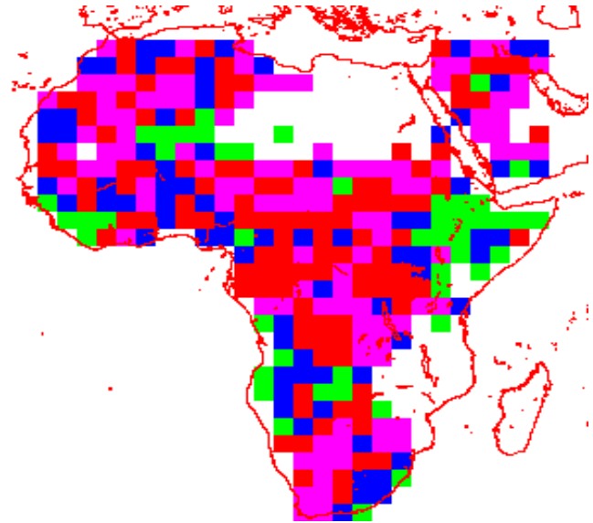
Fig. 8b. Post-onset period: Spatial repartition of the four classes computed by non supervised classification. Same color code as in Fig. 8a.
