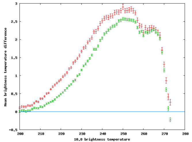
Fig. 2b. Difference of the mean value of 6.2\ \mu\text{m} and 7.3\ \mu\text{m} channels between non rainy and rainy pixels plotted versus 10.8\ \mu\text{m} brightness temperature in red and green, respectively. Curves are plotted with error-bars. Both scales are in Kelvin.
