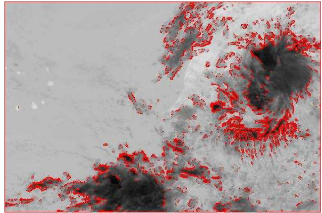
Fig. 3. The 5% highest local variance values are plotted in red on the 8.7\ \mu\text{m} channel image ( 20^\circ\text{N} – 11^\circ\text{N} / 26^\circ\text{W} – 12^\circ\text{W} ). The local variance has been computed on a 3\times 3 window.
