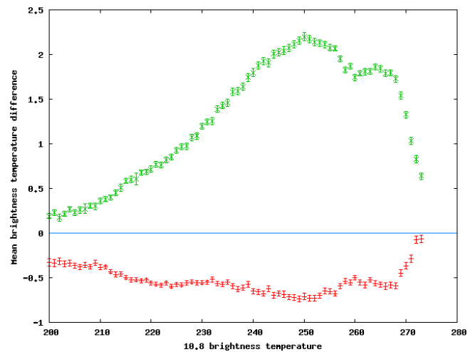
Fig. 2c. Difference of the mean value of 9.7\ \mu\text{m} and 13.4\ \mu\text{m} channels between non rainy and rainy pixels plotted versus 10.8\ \mu\text{m} brightness temperature in red and green respectively. Curves are plotted with error-bars. Both scales are in Kelvin.
