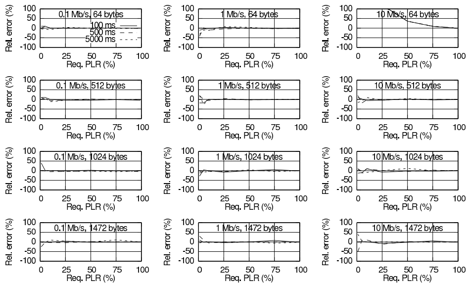
Figure 21: Relative packet loss accuracy error.
