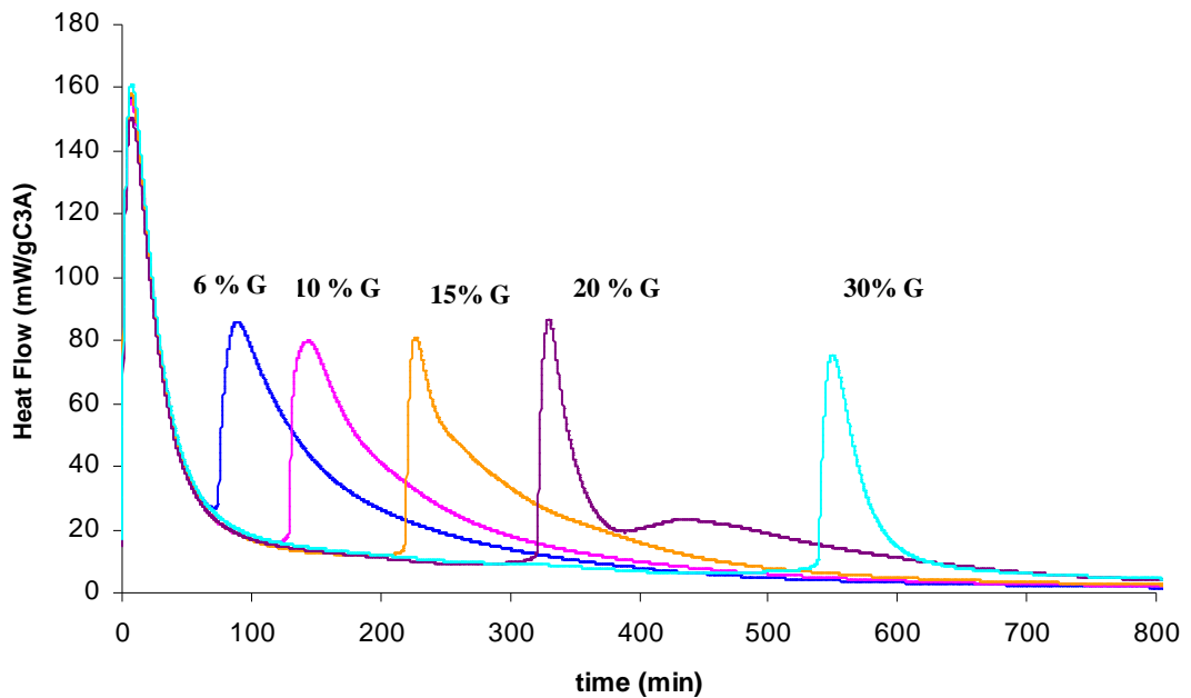
202 Figure 4 : Heat flow evolution over time during C 3 A-gypsum hydration with 203 different initial amount of gypsum (% by weight of C 3 A) in saturated calcium 204 hydroxide solution L/S=25.
