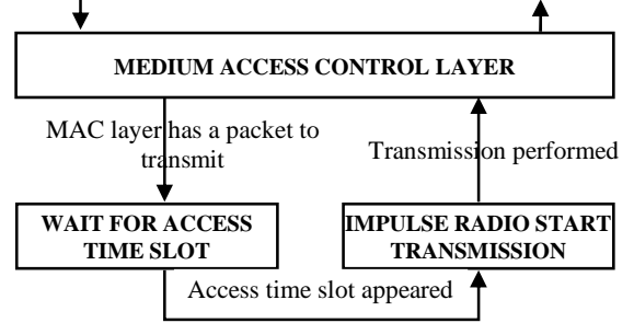
Figure 2: Transmission process.
