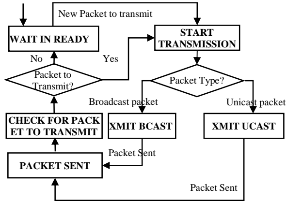
Figure 4: Unslotted-TH illustration.
