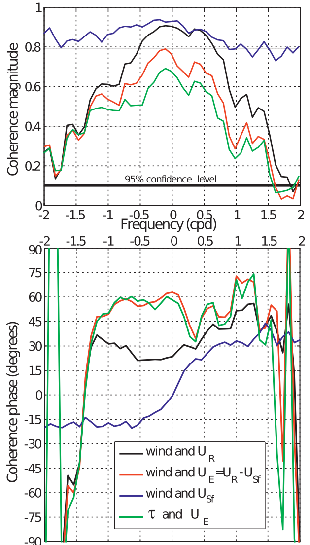
FIG. 4. (a) Magnitude and (b) phase of rotary cospectra of the wind and wind stress with the radar-derived current, Stokes drift, and Eulerian current. The number of degrees of freedom is 108 at the spectral resolution of 0.09 cpd. Coherence is significant at the 95% confidence level for a value of 0.1. Negative and positive frequencies are CW and counterclockwise polarized motions, respectively.
