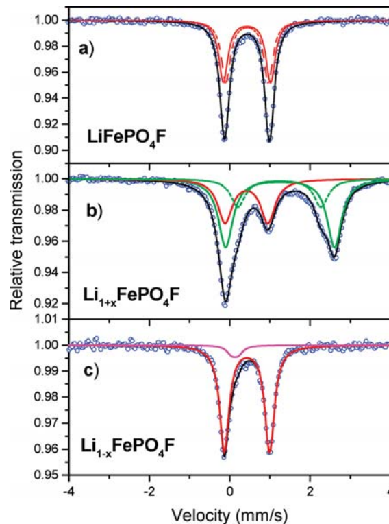
Figure 4. 57 Fe Mössbauer spectra of LiFePO 4 F (a), Li 1+x FePO 4 F ( x \approx 0.8 ) (b) and Li 1-x FePO 4 F ( x \approx 0.1 ) (c).
