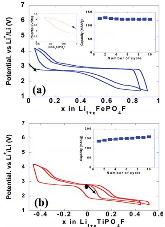
Figure 3. Voltage–composition curve for (a) \text{Li}/\text{LiFePO}_4\text{F} and (b) \text{Li}/\text{LiTiPO}_4\text{F} cells using ionothermally made positive electrodes, together with their corresponding cycling capacity retention as inset. The cells were cycled at a C/15 rate. The voltage–composition curve for a \text{LiFePO}_4\text{F} , which has been started toward oxidation, under the same C/15 current conditions, is shown as an inset in (a).
