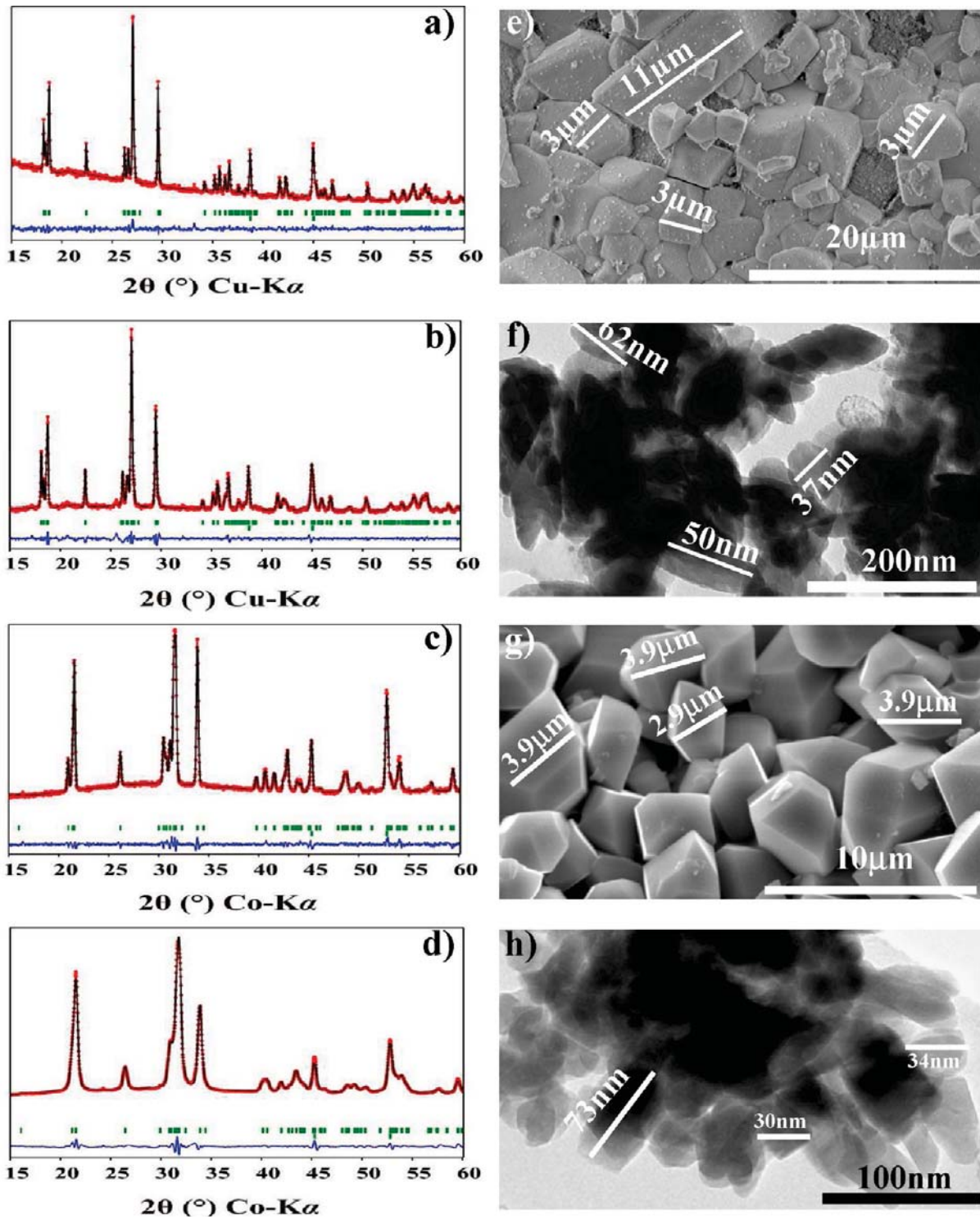
Figure 1. XRD powder patterns for the \text{LiFePO}_4\text{F} and \text{LiTiPO}_4\text{F} phases prepared by the ceramic (a, c) and ionothermal (b, d) processes, respectively, together with their corresponding morphology as deduced by SEM (e, g) and TEM (f, h).
