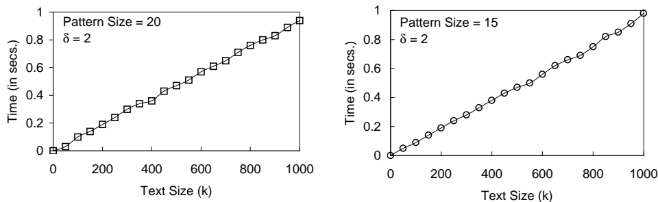
Fig. 2. Timing curves for the SHIFT-AND Procedure.
