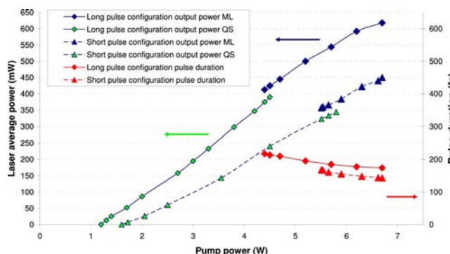
Fig. 6. (Color online) Output average power and pulse duration versus pump power.
