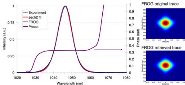
Fig. 3. (Color online) Spectra (left) and spectral phase for the 143 fs pulses directly measured with a spectrometer, retrieved from a SHG FROG (right) and fitted.
