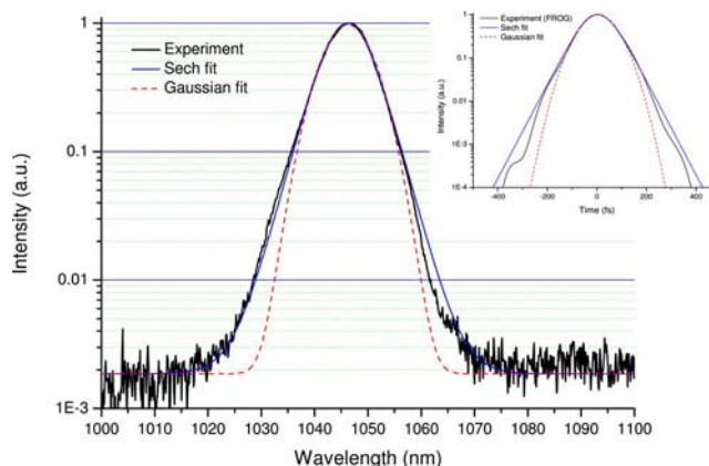
Fig. 4. (Color online) Spectrum and temporal shape comparisons with the sech 2 and the Gaussian shapes.
