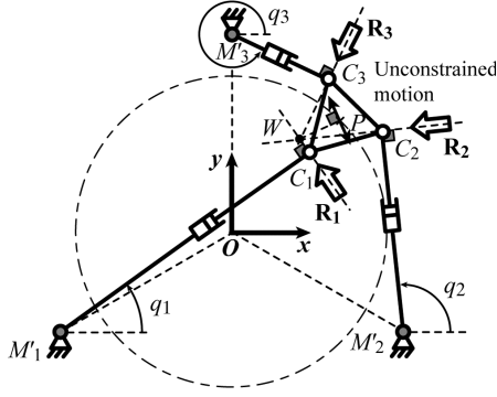
Fig. 3. Type 2 singular configuration of examined manipulator (horizontal projection of the examined structure).
