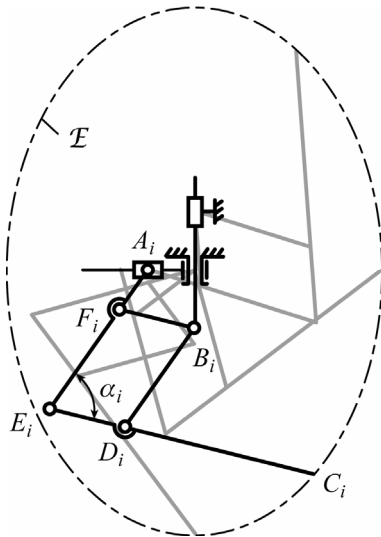
Figure 7. Displacement of C_i when \alpha_i is fixed.
