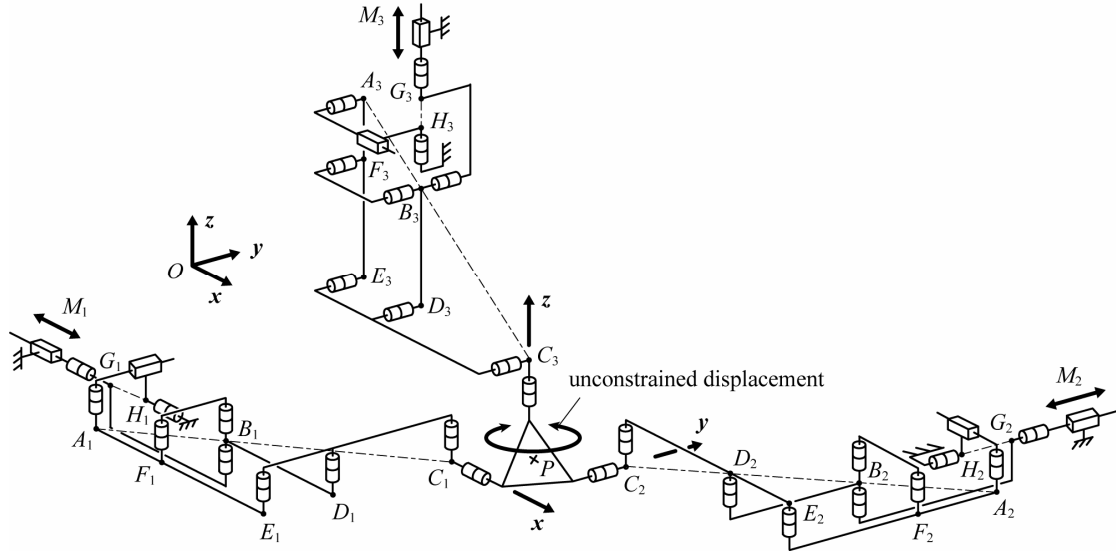
Figure 5. Example of a constraint singularity.
