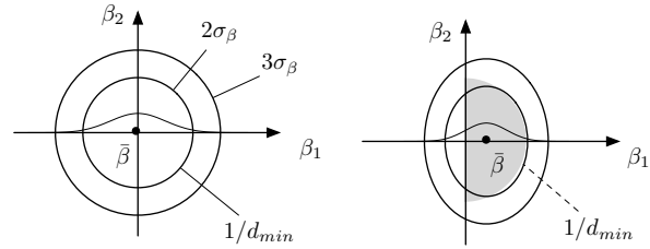
(a) Isotropic Gaussian pdf with \beta (b) Non-isotropic pdf penalizing lines at negative depths.
