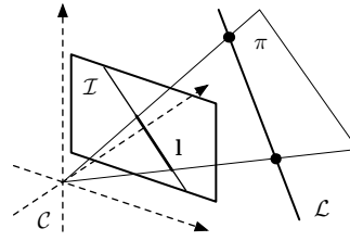
(b) The back-projection of a segment \mathbf{l} gives place to a semi-infinite plane \pi where the line landmark \mathcal{L} must lie. There are 2 unmeasured DOF: the line's depth and its orientation in \pi . The camera gains parallax by moving away from the plane \pi .
