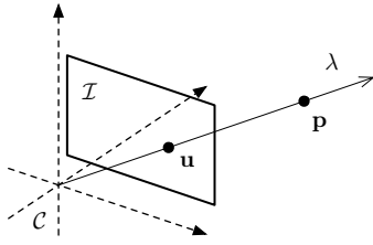
(a) The back-projection of a point \mathbf{u} gives place to a semi-infinite line \lambda where the point landmark \mathbf{p} must lie. There is 1 unmeasured DOF: the point's depth or distance. To observe it, the camera needs to gain parallax by moving away from the line \lambda .
