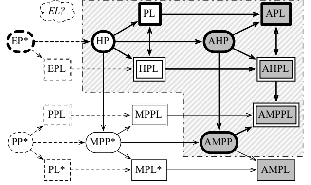
Figure 6. Links between all proposed parametrizations and more. Round boxes are points; square boxes are lines. Single-stroke square boxes are directly-coded lines. Double-stroke square boxes are point-supported lines. Gray boxes are anchored parametrizations. Arrows indicate the links that we established within the discourse. The dashed area encloses all parametrizations benchmarked in this paper. Some other possible parametrizations, in thin line, have not been studied here (there are some repeated acronyms): polar point (PP, i.e. , [\varepsilon, \alpha, d] ), modified-polar point (MPP, [\varepsilon, \alpha, \rho] ); the point-supported Euclidean-points line (EPL, [x_1, y_1, z_1, x_2, y_2, z_2] ), polar-points line (PPL, [\varepsilon_1, \alpha_1, d_1, \varepsilon_2, \alpha_2, d_2] ), and modified-polar-points line (MPPL); and the directly-coded polar line (PL, [\phi, \varepsilon, \alpha, d] ), modified-polar line (MPL, [\phi, \varepsilon, \alpha, \rho] ), and anchored modified-polar line (AMPL). There is no such thing as a directly-coded Euclidean line (EL). Dashed-stroke elements do not benefit from the inverse-distance property and are not suited for undelayed initialization. Minimal parametrizations are marked with an asterisk.
