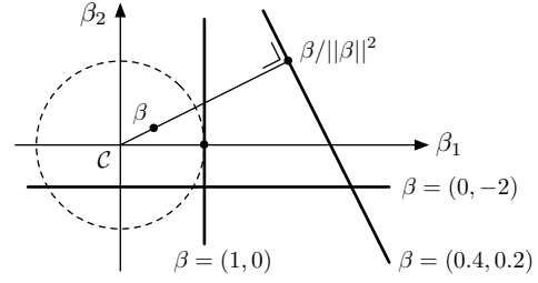
Figure 4. Different lines in the representation plane \pi (see Fig. 3(b)) in camera frame \mathcal{C} , as a function of \beta . The circle is of unit radius. Given \beta , the line is such that its closest point to \mathcal{C} is \beta/\|\beta\|^2 . The line is orthogonal to the vector \beta . See also Fig. 9.
