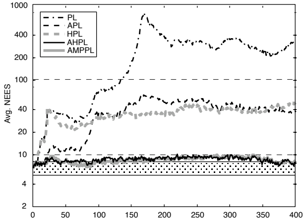
Figure 22. Consistency of PL, APL, HPL, AHPL and AMPPL. Average NEES over 25 runs for 400 frames (one turn around the house). Plücker-based lines (PL and APL) do not behave consistently, even when anchored. Lines based on homogeneous points (HPL) neither, as expected from the HP behavior. Anchored point-supported lines (AHPL and AMPPL) behave similarly and close to consistency.
