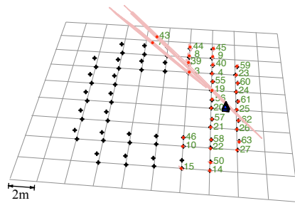
Figure 16. Simulated 3D environment for benchmarking 3 point parametrizations.
