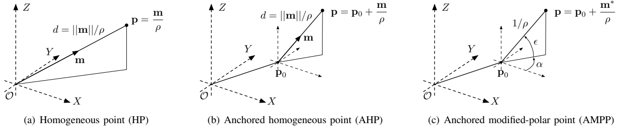
Figure 2. Point parametrizations. Homogeneous and anchored homogeneous do not require \mathbf{m} to be a unit vector. In modified-polar point, the observed ray is coded by two angles: the derived direction vector is unitary and hence \rho is exactly inverse-distance. The anchor point \mathbf{p}_0 in AHP and AMPP corresponds to the optical center at initialization time.
