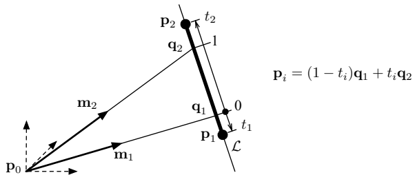
Figure 13. Segment endpoints in the local ordinate frame of point-defined lines HL, AHL and AMPL. The line is supported by two points \mathbf{q}_i = \mathbf{p}_0 + \mathbf{m}_i / \rho_i . The local frame has its origin at \mathbf{q}_1 and the unit length and positive orientation are defined by \mathbf{q}_2 - \mathbf{q}_1 . The endpoint \mathbf{p}_i is coded by the scalar abscissa t_i , satisfying \mathbf{p}_i = (1 - t_i)\mathbf{q}_1 + t_i\mathbf{q}_2 . Only the abscissas t_i are stored.
