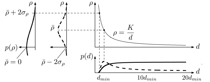
Figure 7. Inverse-distance pdf . A Gaussian p(\rho) = \mathcal{N}(\rho - \bar{\rho}, \sigma_\rho^2) is defined in inverse-distance (vertical axes). We have ample choice: in one extreme (dashed) we may define it so that \bar{\rho} - 2\sigma_\rho = 0 ; the other extreme (solid) takes \bar{\rho} = 0 . In all cases, we have (\bar{\rho} + 2\sigma_\rho) = K/d_{min} . They result in pdfs in distance (bottom) that cover from a minimal distance d_{min} to infinity. K is just a proportionality constant, e.g. K = 1 for AMPP, and K = \|\mathbf{K}^{-1}\underline{\mathbf{u}}\| for AHP and HP. We can also normalize \mathbf{K}^{-1}\underline{\mathbf{u}} at initialization time and take K = 1 , in which case \rho is exactly equal to inverse-distance.
