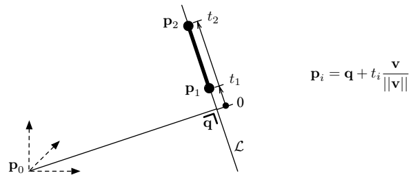
Figure 12. Segment endpoints in the local ordinate frame of Plücker-based lines PL and APL. The closest point \mathbf{q} to the anchor is the local origin, and the unit length and positive orientation are defined by a normalized director vector \mathbf{u} = \mathbf{v} / \|\mathbf{v}\| . The endpoint \mathbf{p}_i is coded by the scalar abscissa t_i , satisfying \mathbf{p}_i = \mathbf{q} + t_i \mathbf{v} / \|\mathbf{v}\| . Only the abscissas t_i are stored.
