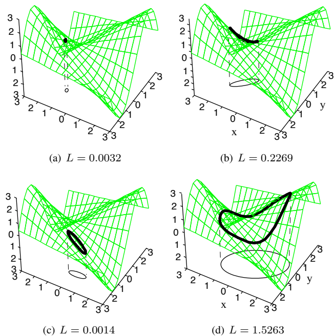
Figure 15. Linearity index L of the MISO function z = f(x, y) = x \cdot \sin(y) for different probability regions. We illustrate the projection (thick black) of the 2-sigma elliptical bound of the probability region (thin black) onto the surface \mathcal{S} = \{(x, y, z) \text{ s.t. } z = f(x, y)\} (mesh). The more elliptic the projected shape, the more linear is the function and smaller the index L . (a) A tiny probability region gives good linearity and a very small index. (b) A large probability region usually obliges the ellipse to bend over the surface, meaning high non-linearity and resulting in a large index. (c) If such a large ellipse falls on a planar region of the surface, the index drops to show good linearity. (d) An extreme case of very high non-linearity.
