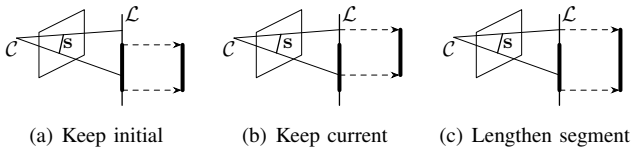
Figure 14. The three general strategies for updating 3D segment endpoints. (a) Endpoints are defined at initialization time and never updated. (b) Endpoints are systematically updated according to the current observation. (c) Endpoints are updated only if this lengthens the 3D segment.
