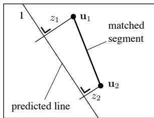
Figure 11. Plücker line observation update. Direct measurement of the innovation \mathbf{z} = (z_1, z_2) as the two signed orthogonal distances from the detected endpoints to the expected (or predicted) line.
