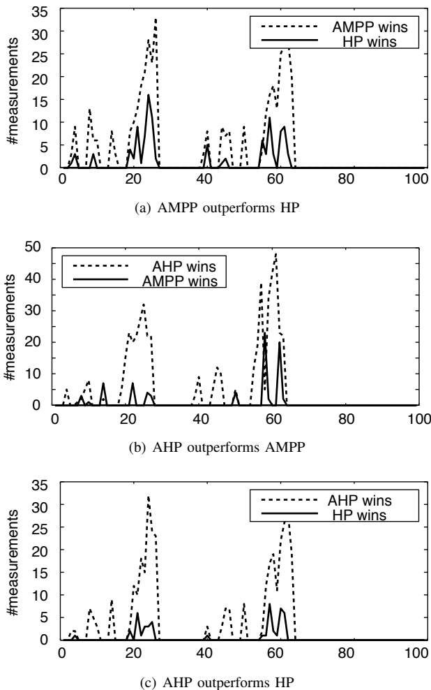
Figure 17. Bi-lateral comparisons of the linearity index for HP, AHP and AMPP. Each plot shows, at each frame, the number of landmarks of one type showing lower linearity index (better linearity) than the other type, and vice versa.
