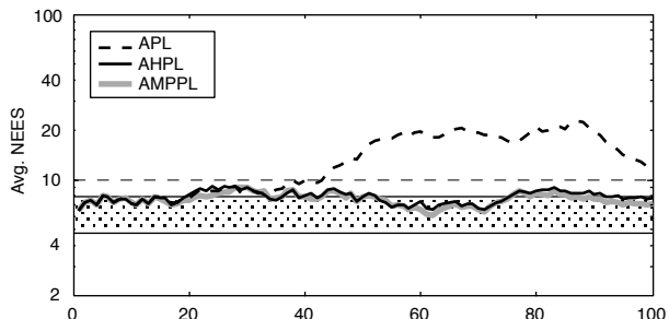
Figure 23. Average NEES over 25 runs for 100 frames (frontal trajectory). Again, only anchored point-supported lines behave close to consistency.
