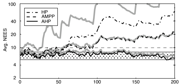
Figure 20. Consistency of HP, AMPP and AHP. Average NEES over 25 runs for 200 frames (1/4 turn) with parameters of Set 2 and 10 initializations in the first frame. Thick gray : initialization with an alternative prior (\bar{\rho}, \sigma_\rho) = (1, 1) .
