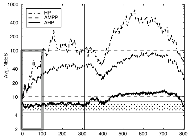
Figure 19. Consistency of HP, AMPP and AHP. Average NEES of the 6-DOF vehicle pose [x, y, z, \phi, \theta, \psi]^T over 25 runs for 800 frames (2 turns) and parameters of Set 1. The dotted horizontal band between abscissas \underline{\epsilon} = 4.719 and \bar{\epsilon} = 7.432 mark the 95% consistency region: the filter is consistent if the average NEES is inside this band. The vertical line marks the loop closure at frame 308. The framed area corresponds to the area covered by Fig. 20.
