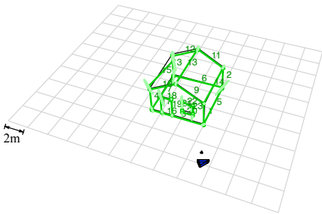
Figure 21. Simulated 3D environment for benchmarking 5 line parametrizations.
