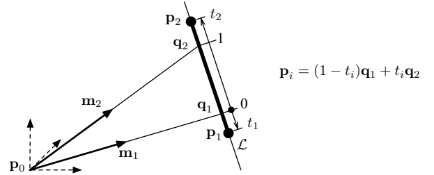
Figure 13. Segment endpoints in the local ordinate frame of point-defined lines HL, AHL and AMPL. The line is supported by two points \mathbf{q}_i = \mathbf{p}_0 + \mathbf{m}_i / \rho_i . The local frame has its origin at \mathbf{q}_1 and the unit length and positive orientation are defined by \mathbf{q}_2 - \mathbf{q}_1 . The endpoint \mathbf{p}_i is coded by the scalar abscissa t_i , satisfying \mathbf{p}_i = (1 - t_i)\mathbf{q}_1 + t_i\mathbf{q}_2 . Only the abscissas t_i are stored.
